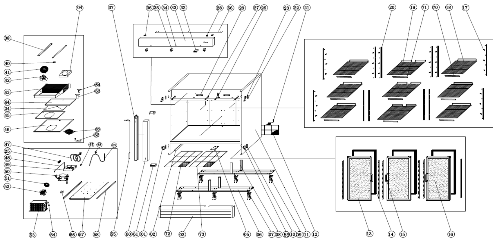
EXPLODED VIEW OF KCHRI81R3GDR
