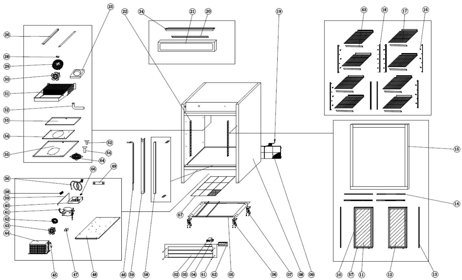
EXPLODED VIEW OF KCHSGM36R
