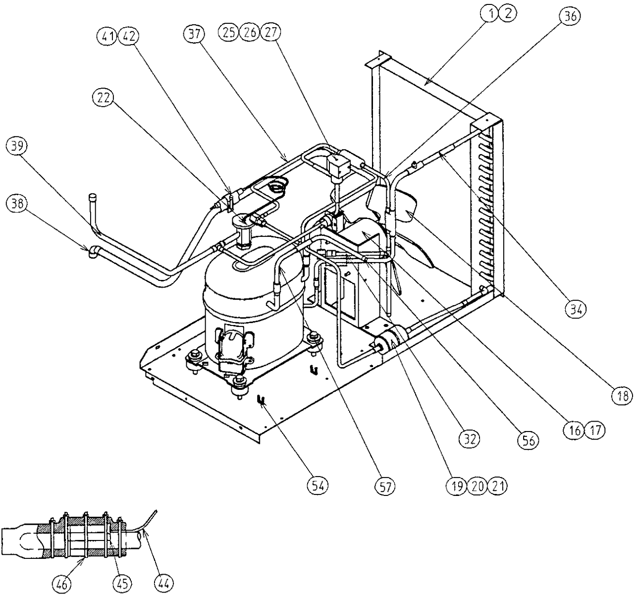
THERMISTOR ATTACHMENT
