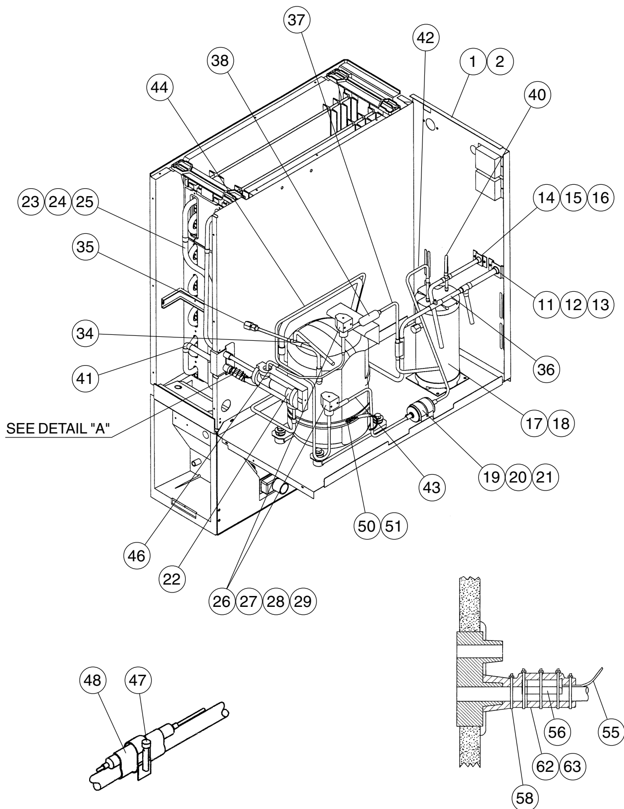
DETAILED HOLDER / EXPANSION VALVE
