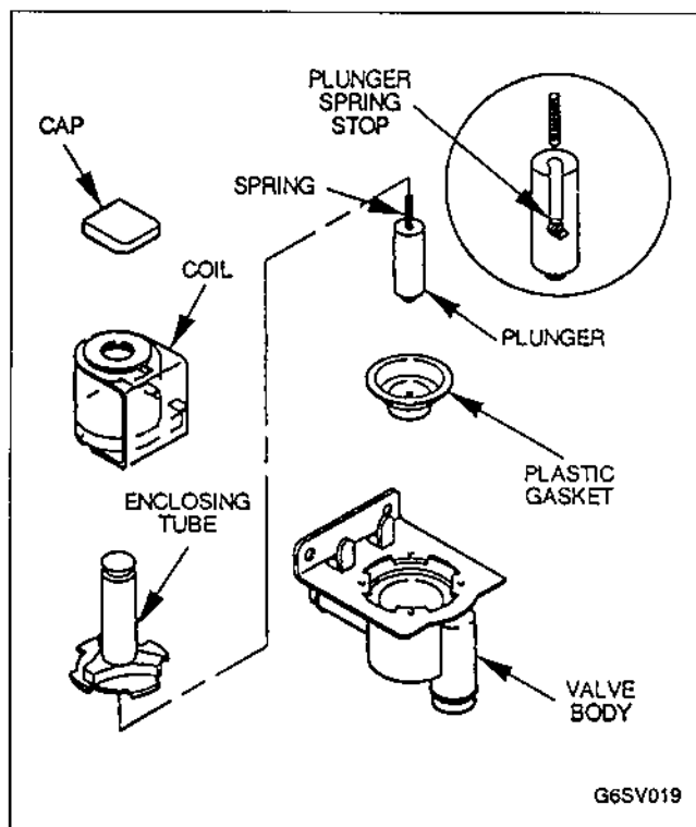
FIGURE 20. PLASTIC BODY WATER DUMP VALVE DISASSEMBLY
