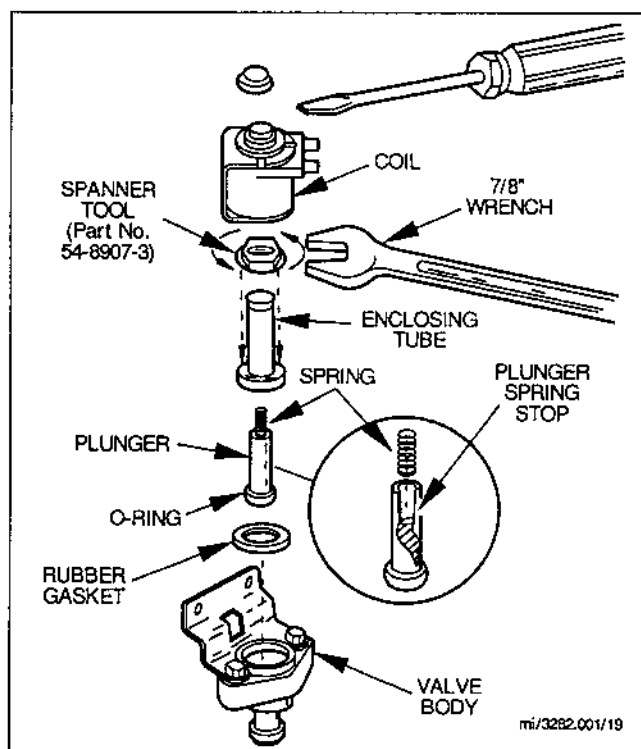
FIGURE 19. BRASS BODY WATER DUMP VALVE DISASSEMBLY
