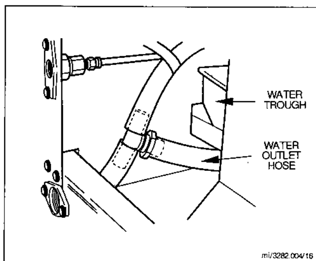
FIGURE 16. DISCONNECT WATER OUTLET HOSE
