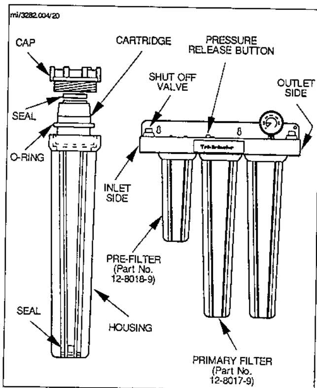
FIGURE 21. WATER FILTRATION
