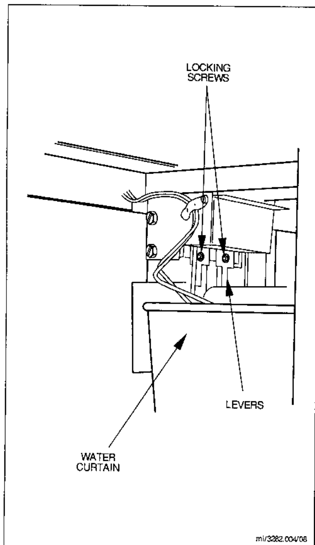
FIGURE 8. BIN SWITCH CHECK
