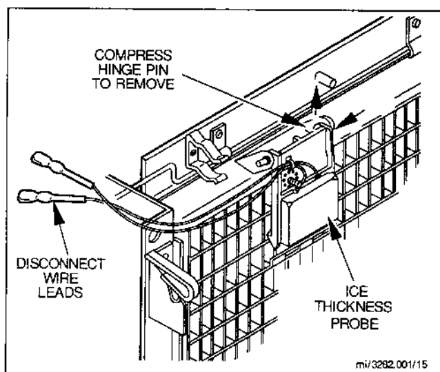
FIGURE 15. ICE THICKNESS PROBE REMOVAL
