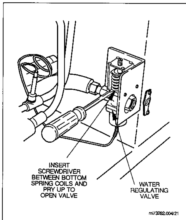
FIGURE 22. MANUALLY OPEN WATER REGULATING VALVE
