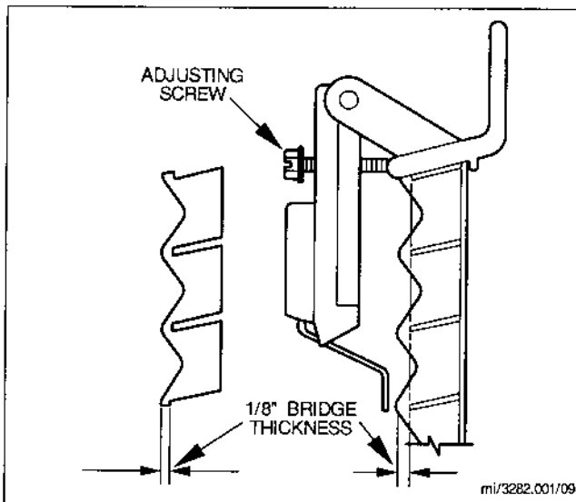
FIGURE 9. ICE THICKNESS CHECK
