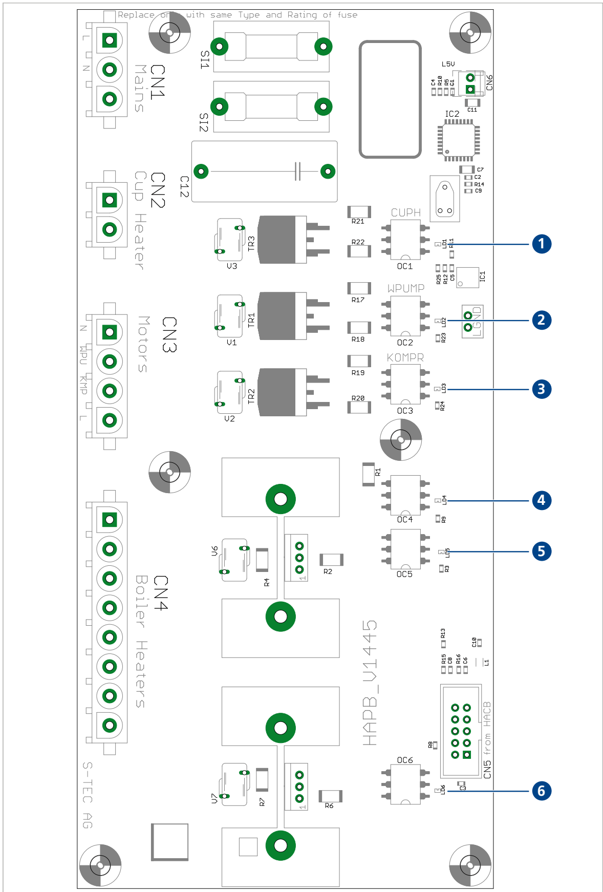
1 LD1: Cup heater
