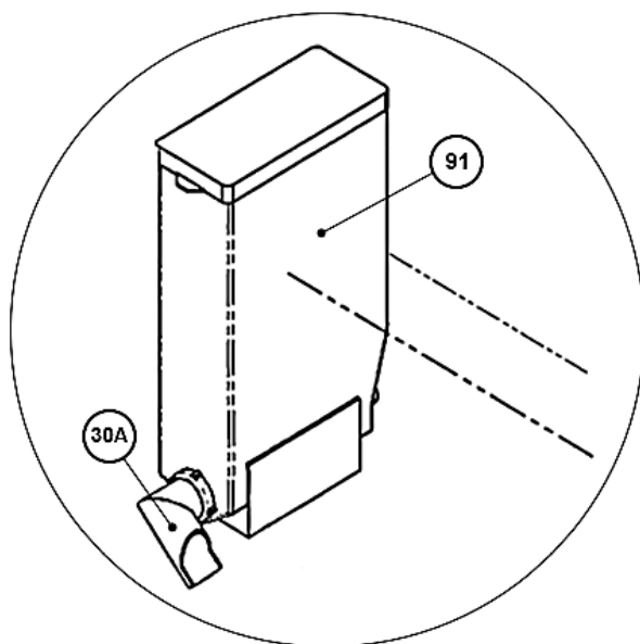
30 LH HOPPER ASSEMBLY
