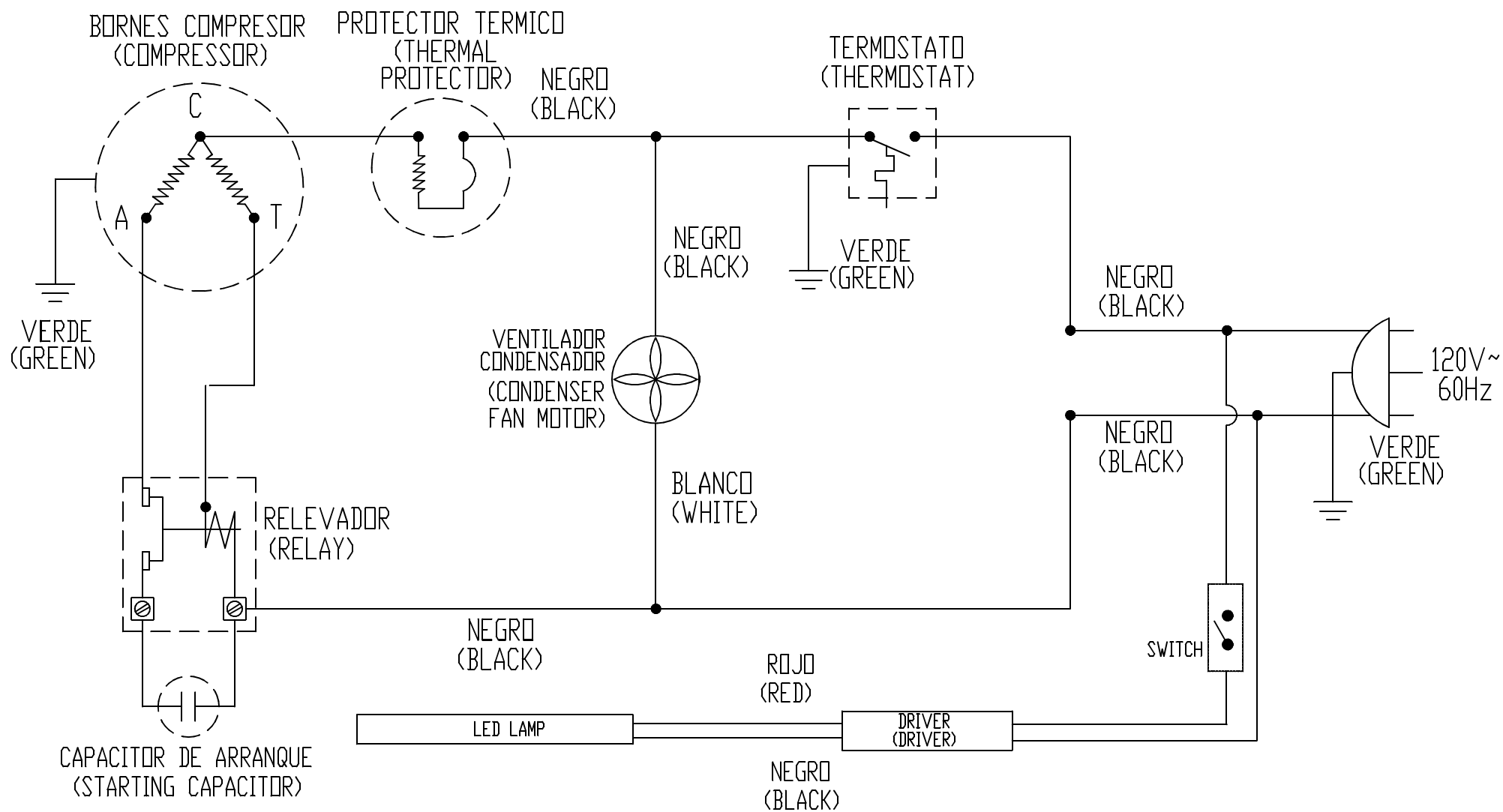
DIAGRAMA ELECTRICO (ELECTRIC DIAGRAM)
