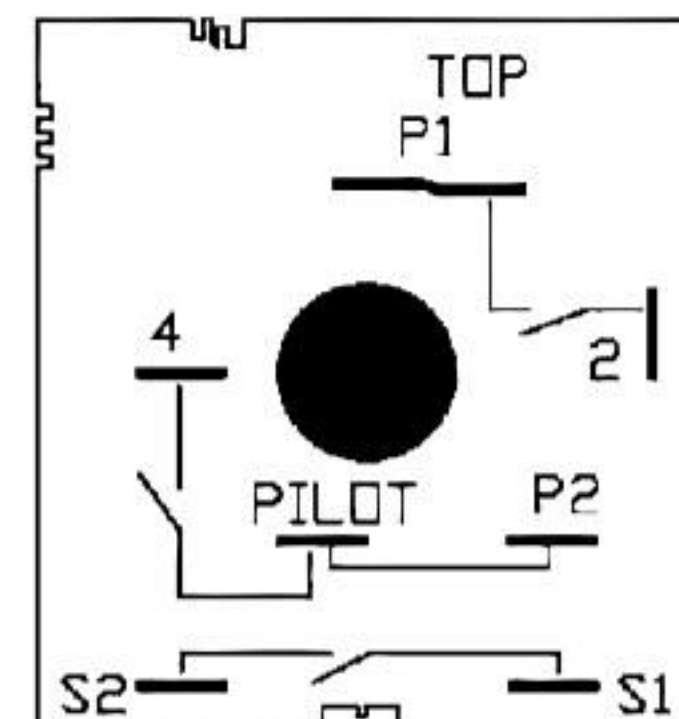
Infinity Switch
