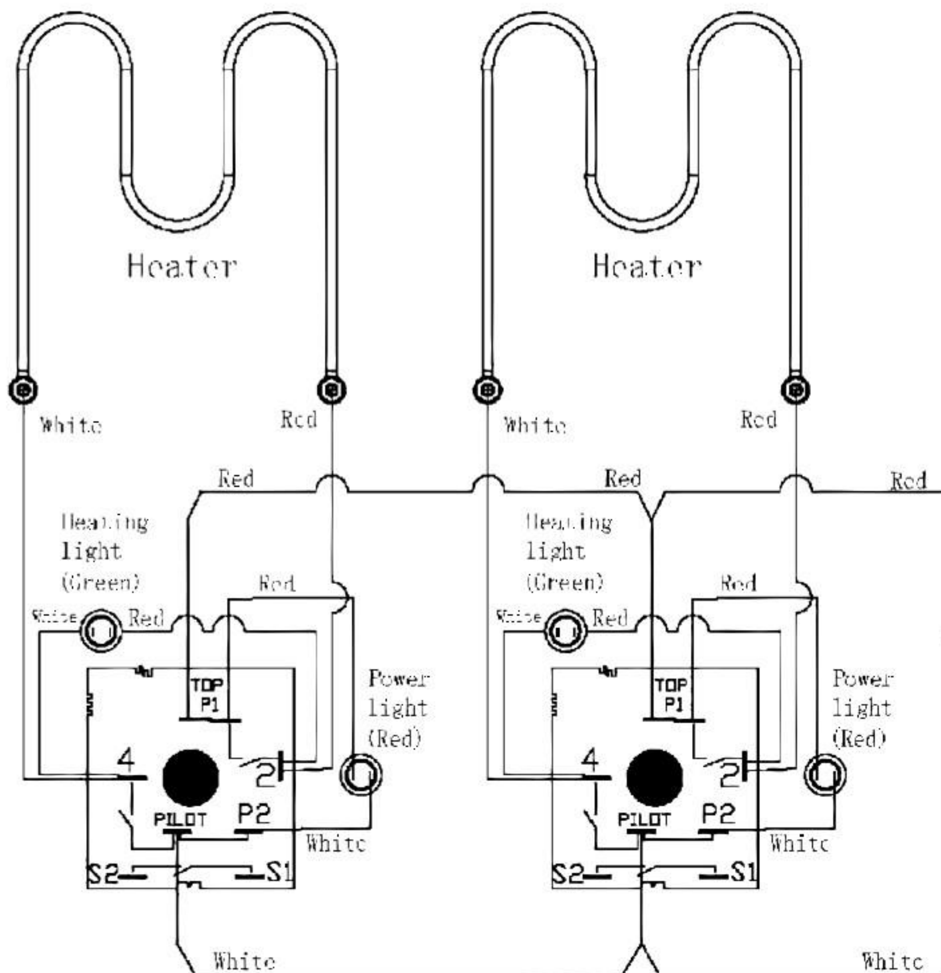
Infinity Switch
