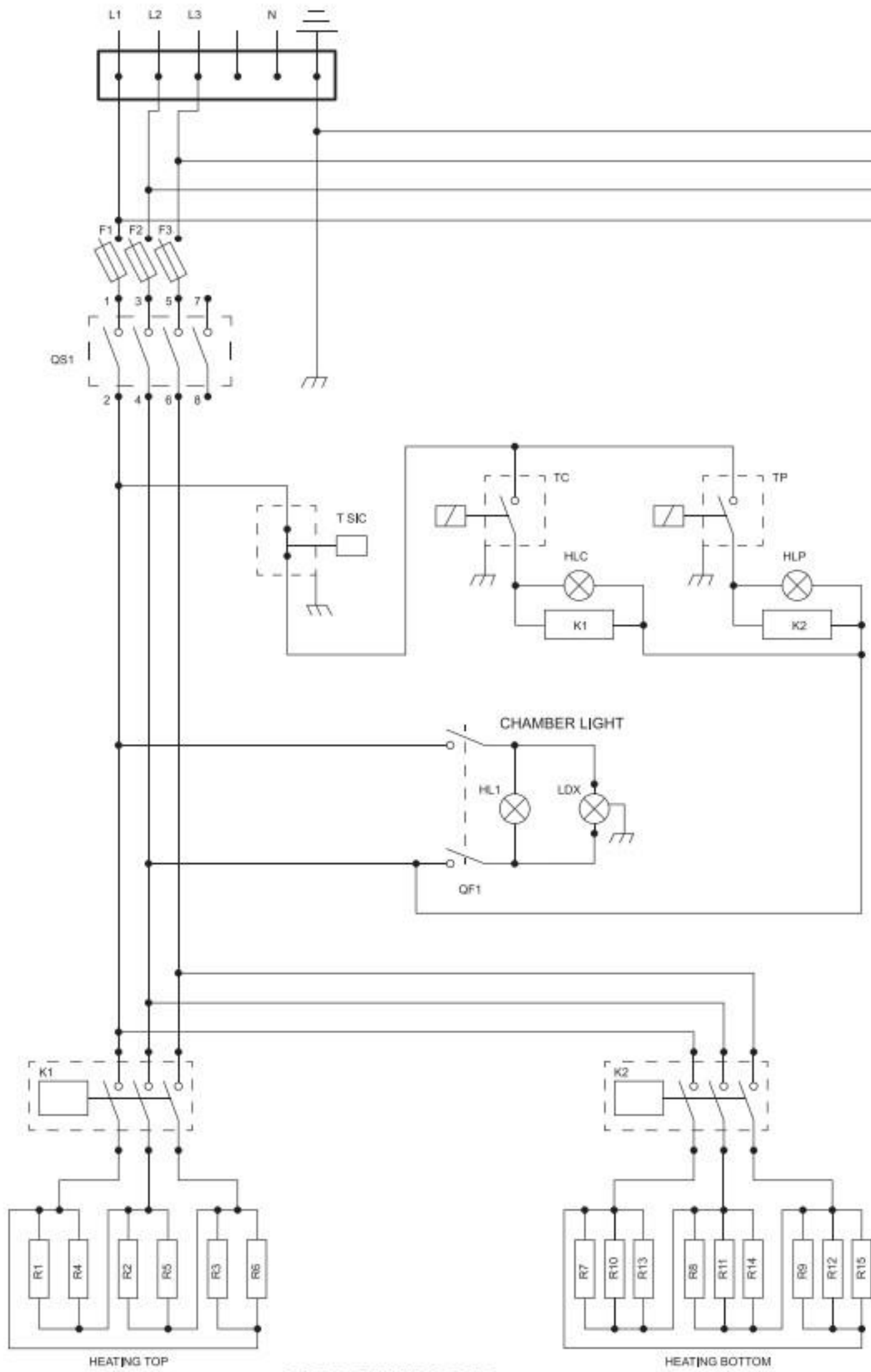
TOP CHAMBER
