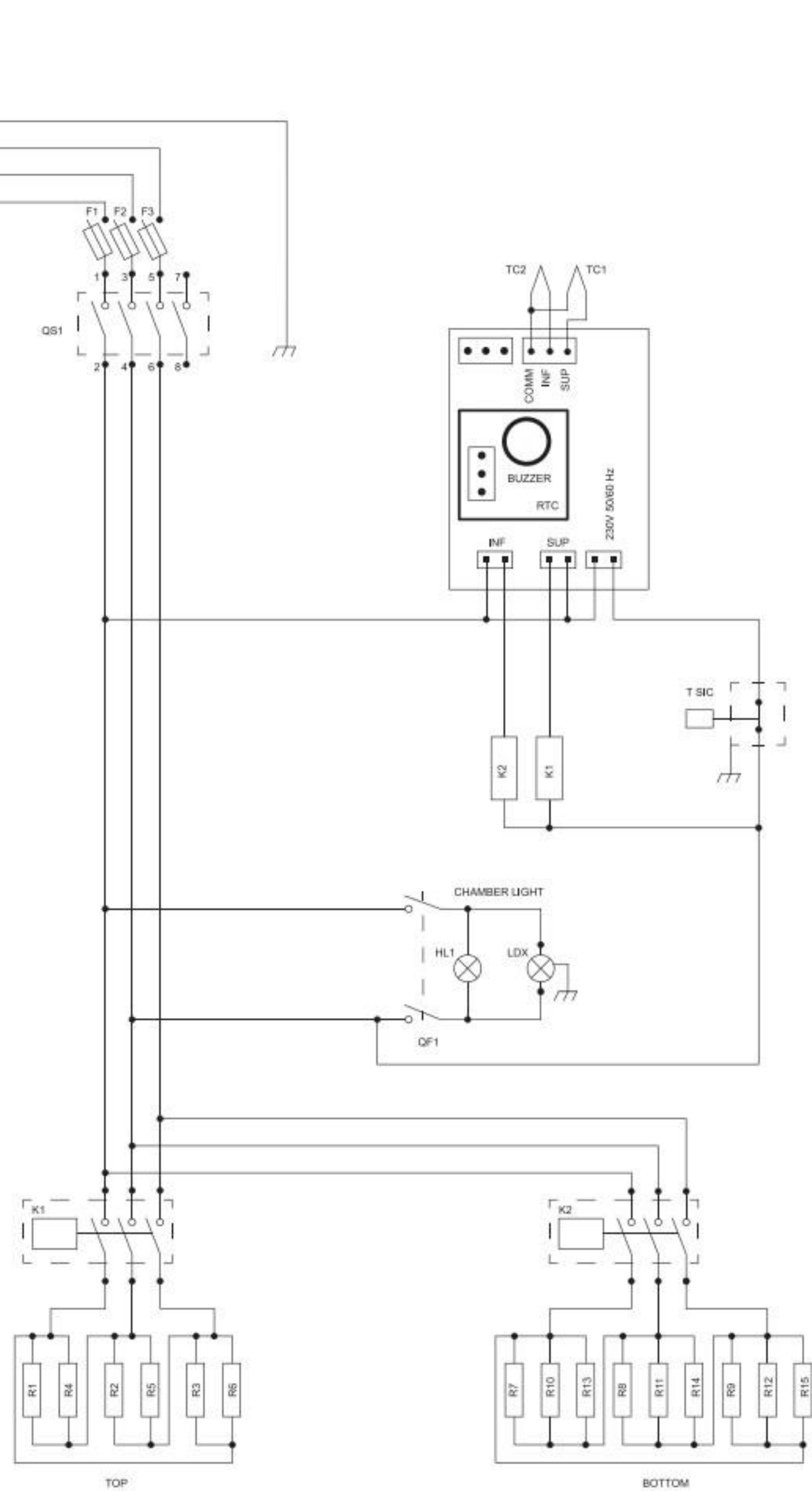
BOTTOM CHAMBER
