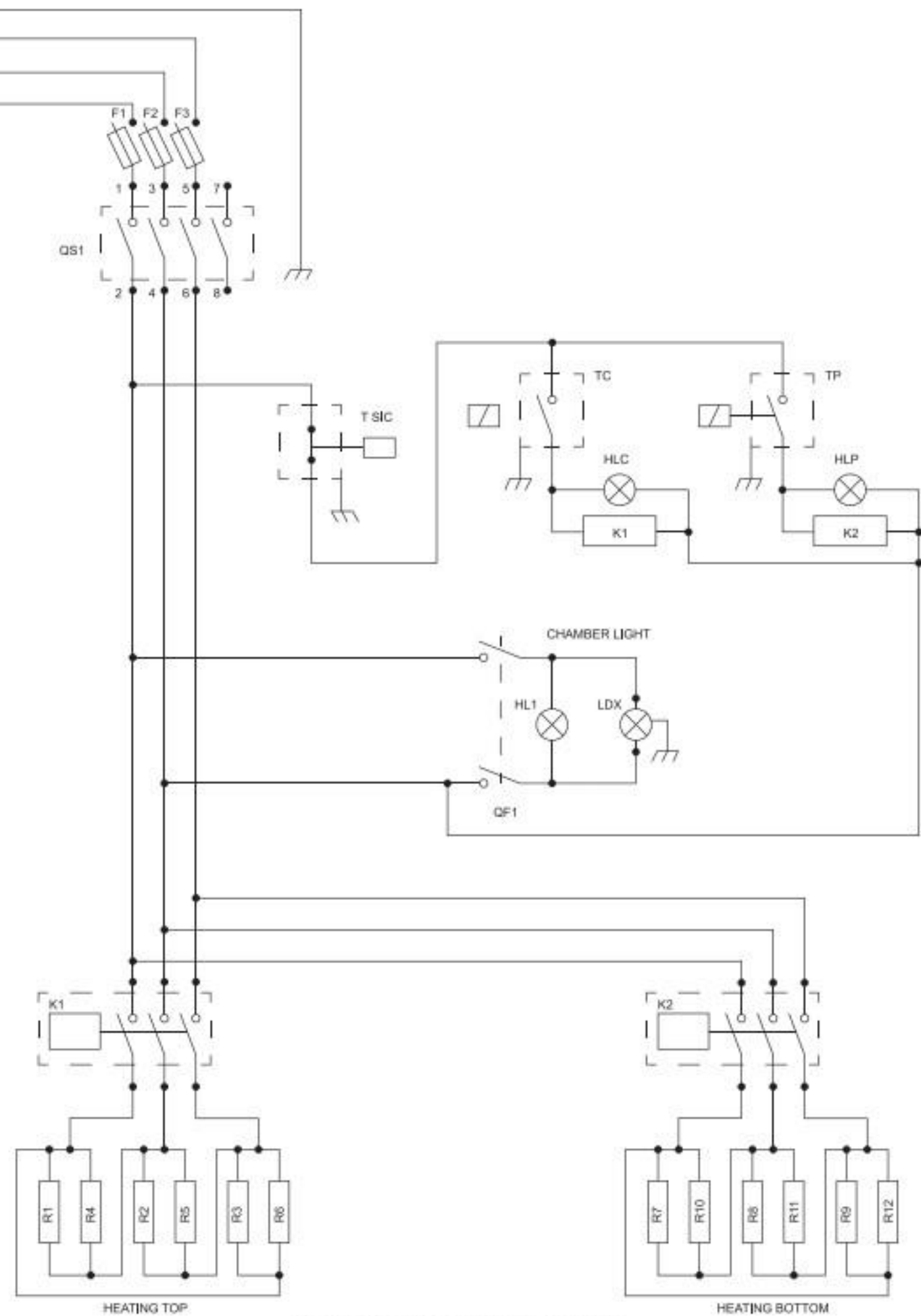
BOTTOM CHAMBER
