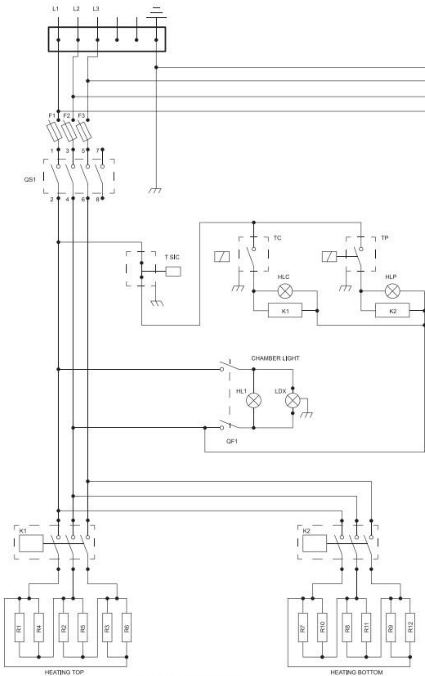
TOP CHAMBER
