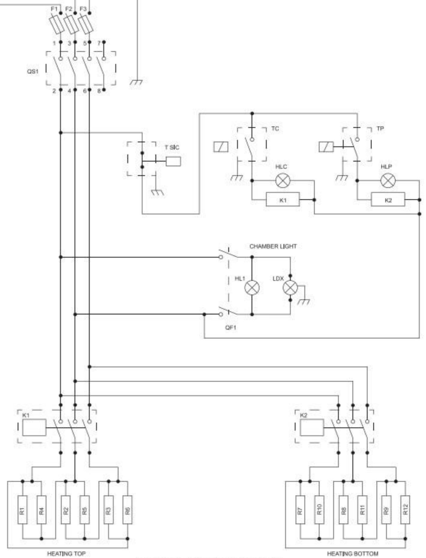
BOTTOM CHAMBER
