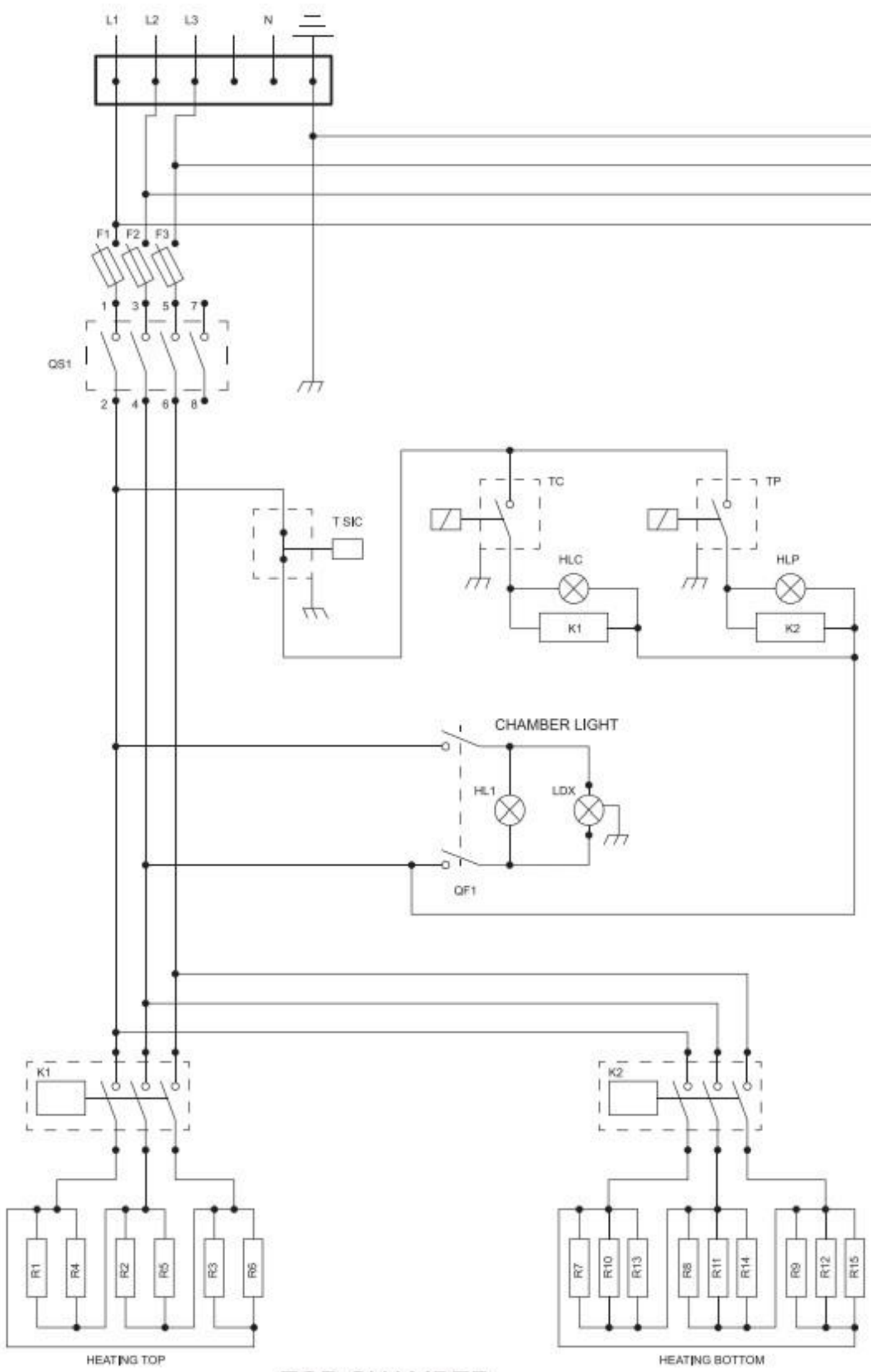
TOP CHAMBER
