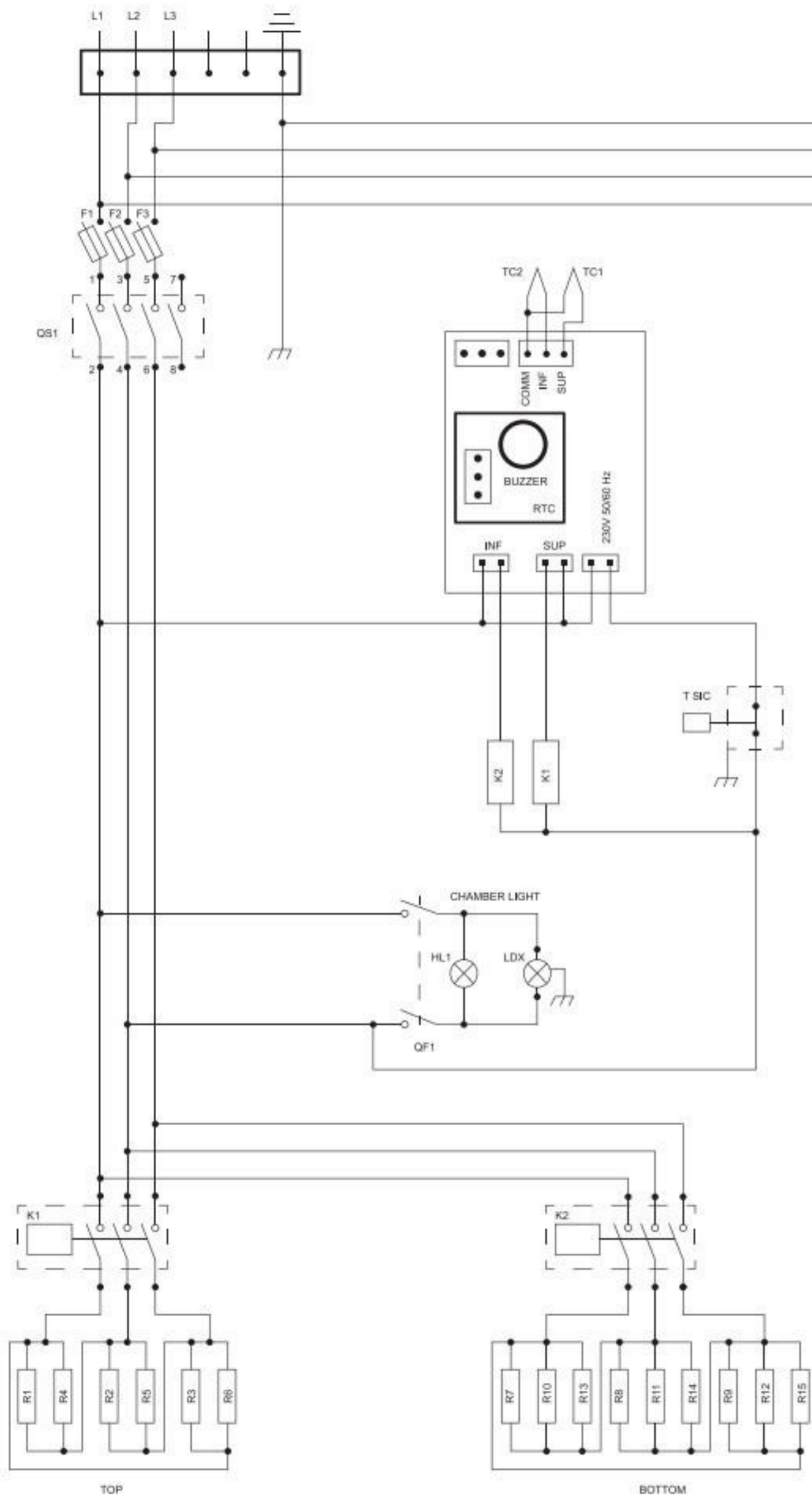
TOP CHAMBER
