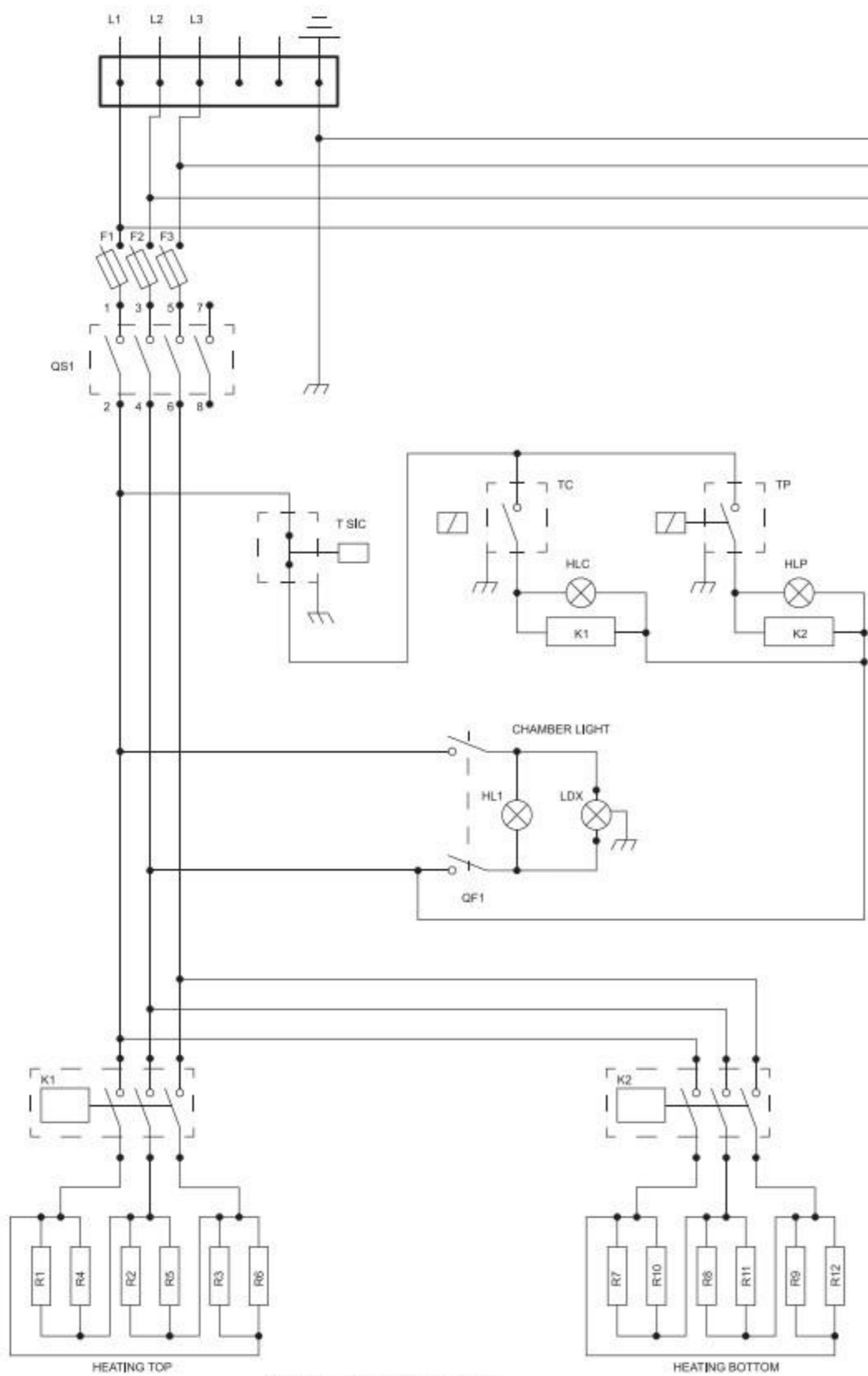
TOP CHAMBER
