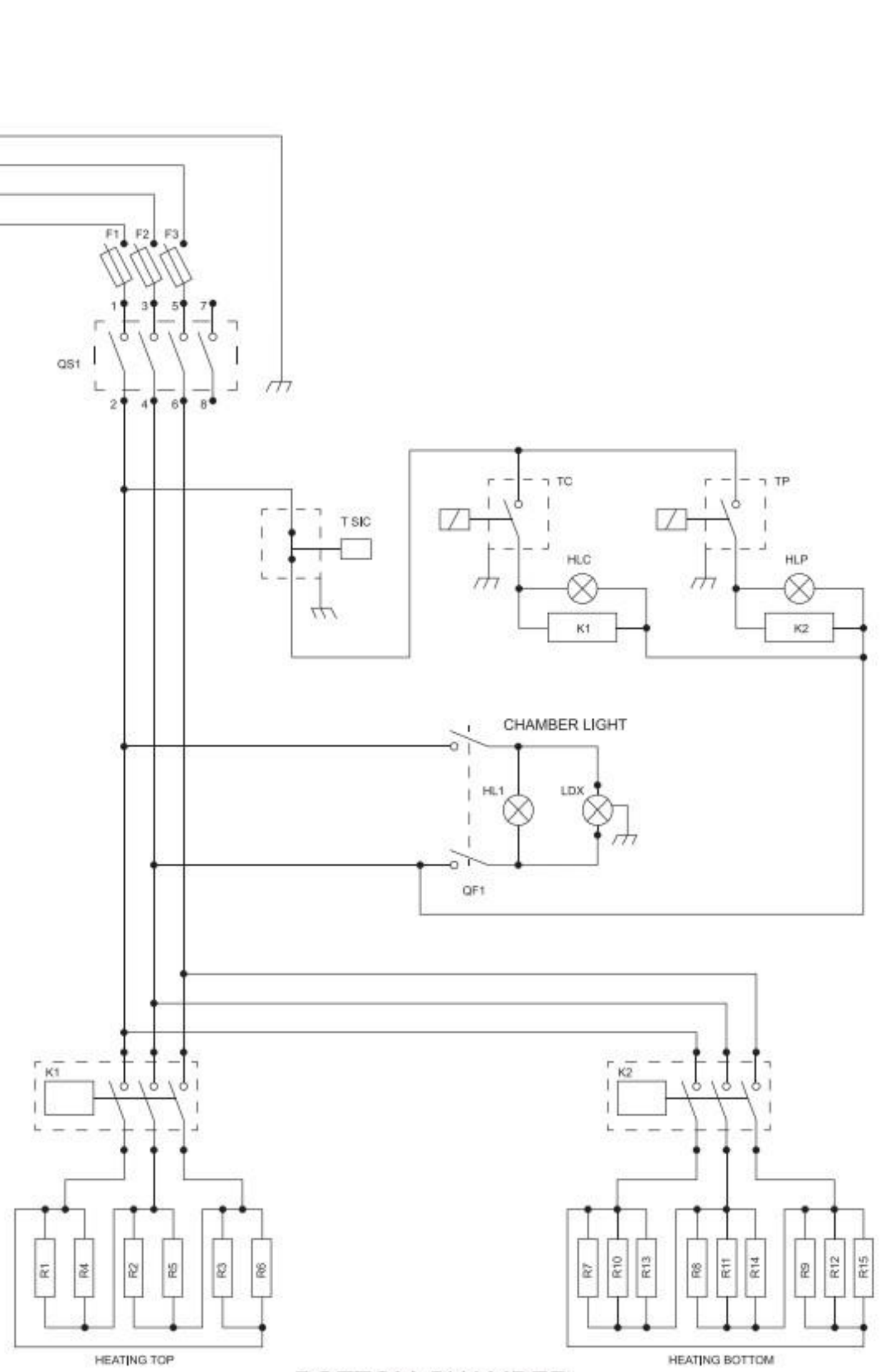
BOTTOM CHAMBER
