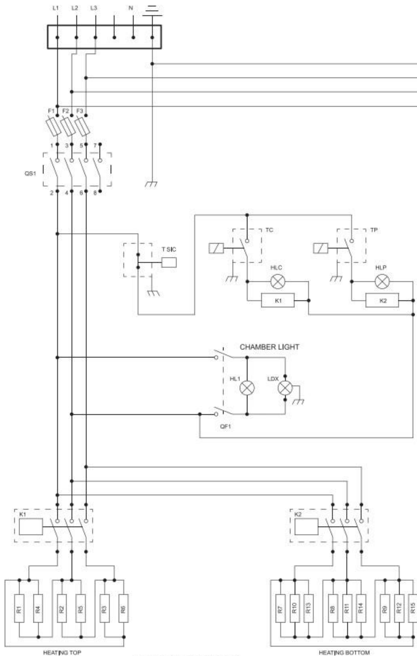
TOP CHAMBER
