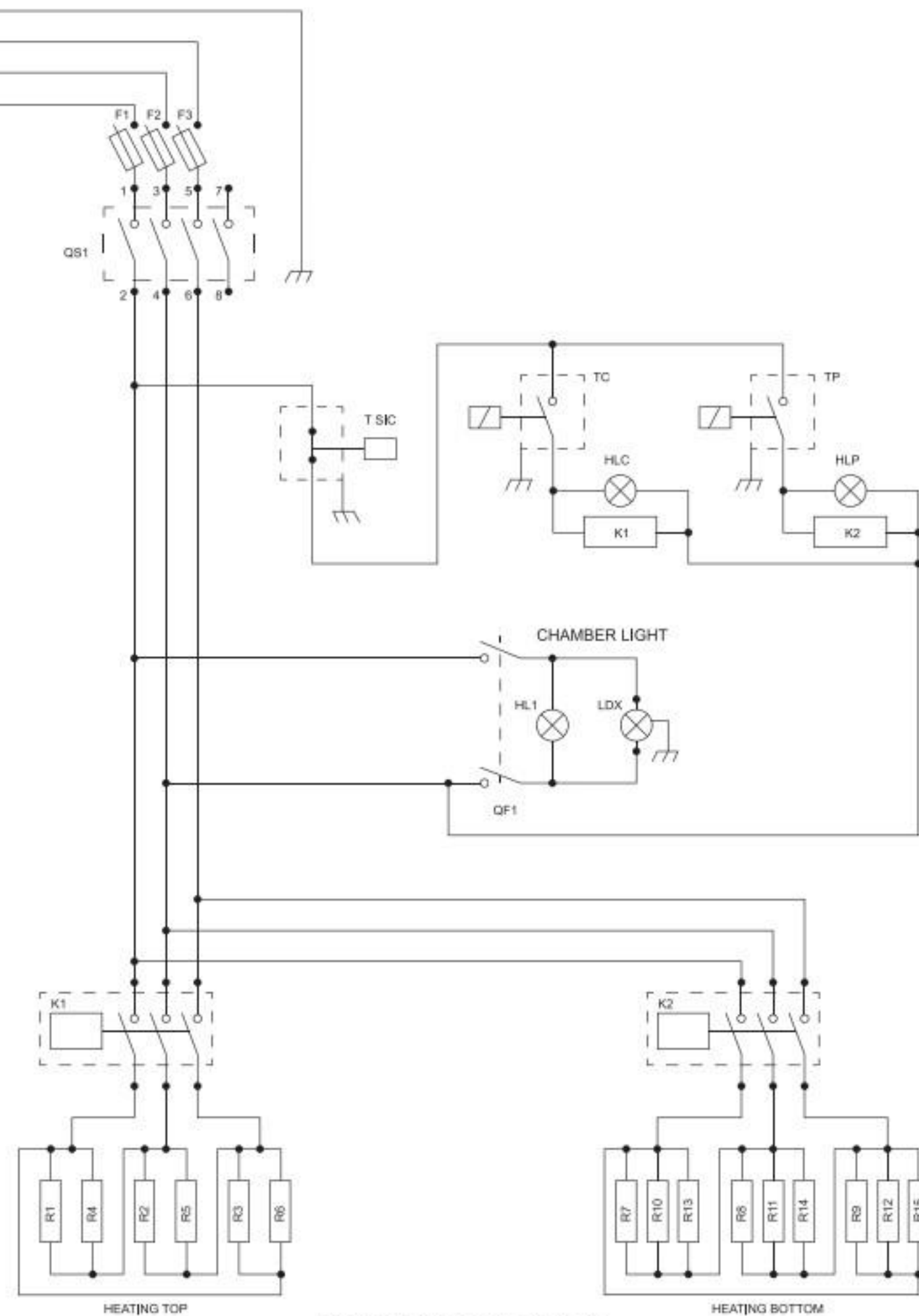
BOTTOM CHAMBER
