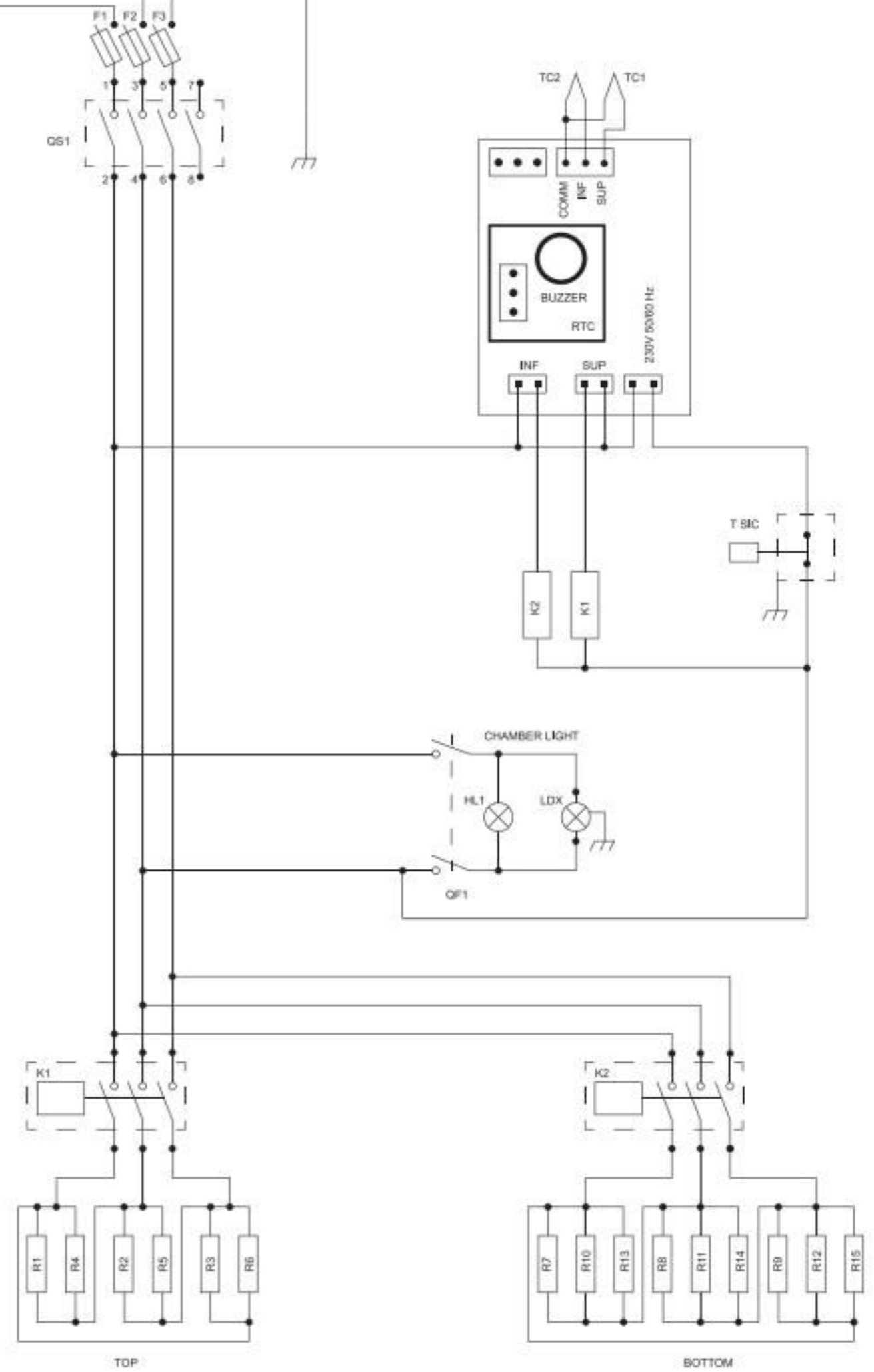
BOTTOM CHAMBER
