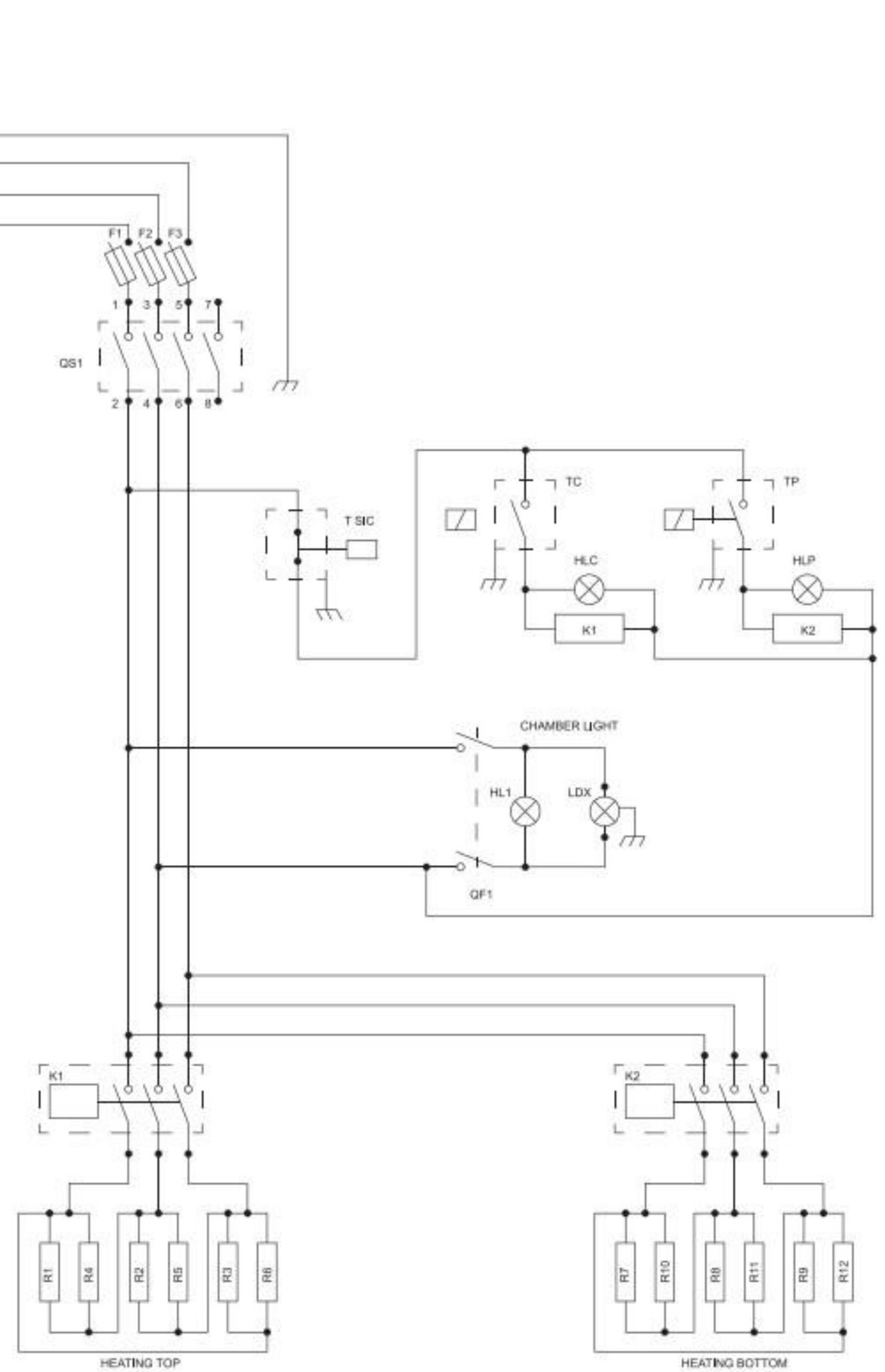
BOTTOM CHAMBER
