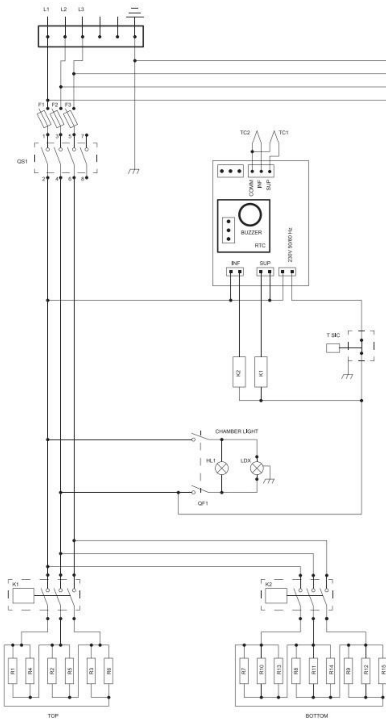
TOP CHAMBER
