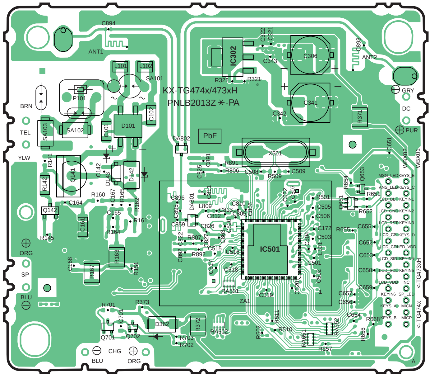
KX-TG4741/4742/4743/4744 CIRCUIT BOARD (Base Unit_Main (Component View))
