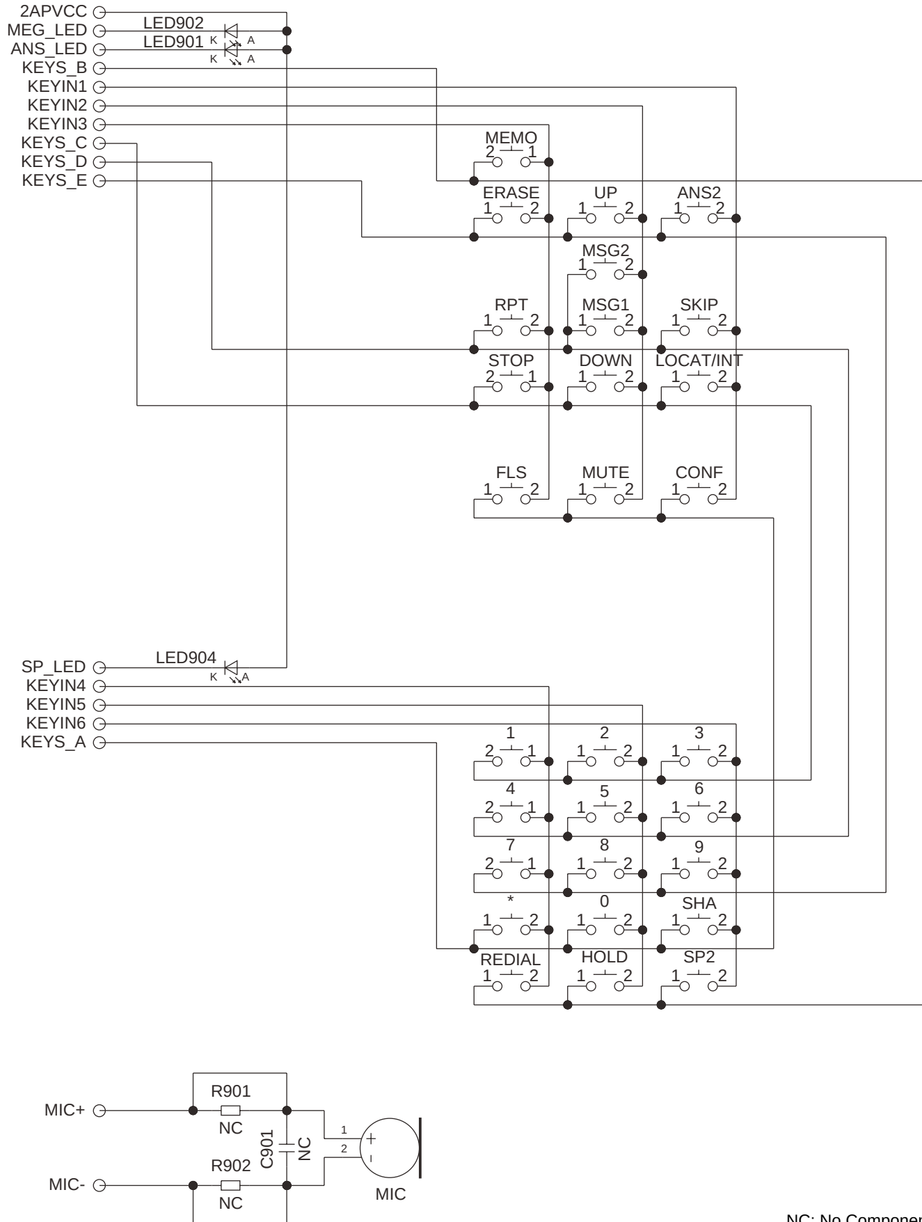
KX-TG6440 SCHEMATIC DIAGRAM (Base unit_Operation)
