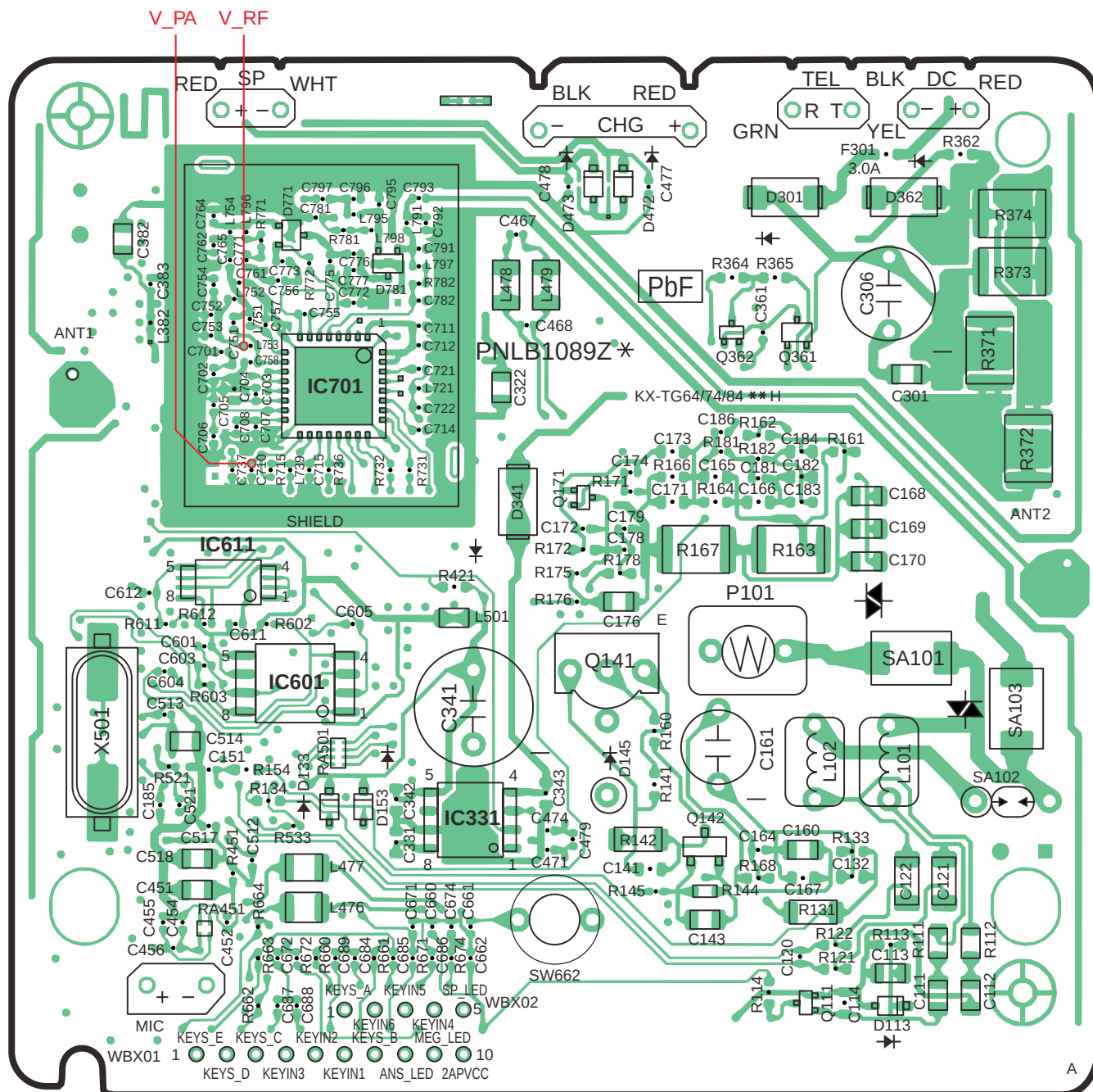
KX-TG6440 CIRCUIT BOARD (Base Unit Main (Component View))
