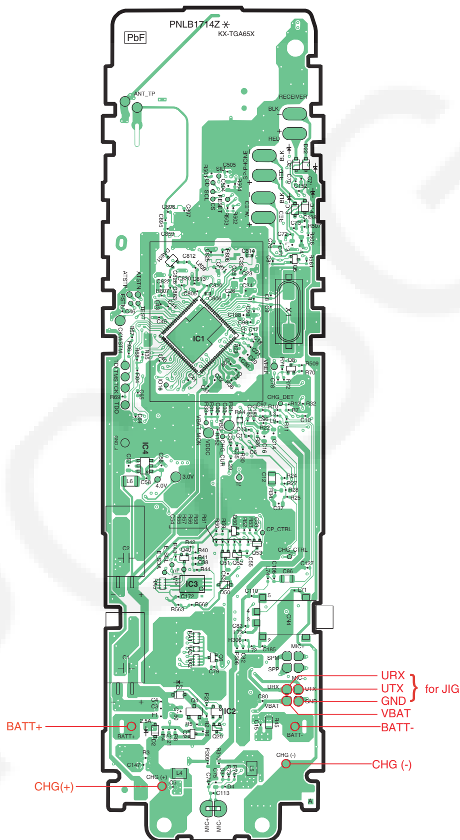
KX-TGA653 CIRCUIT BOARD (Handset_Main (Component View))
