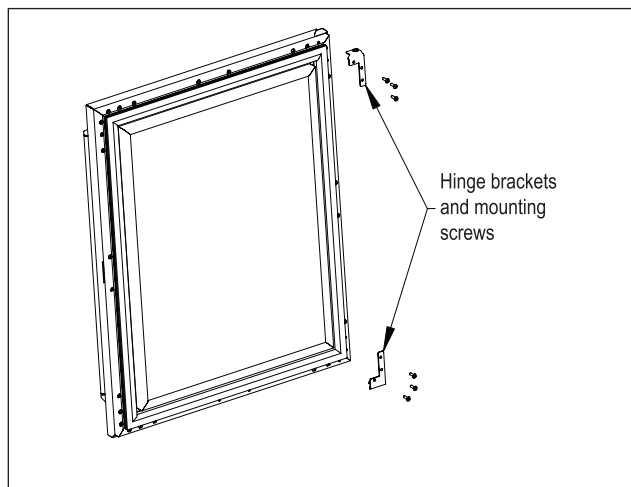
Figure 6: Door Brackets
