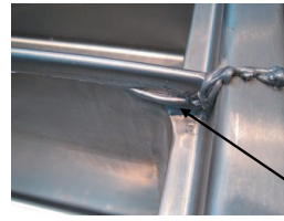
APPLY THE GREY-COLORED NSF APPROVED SEALANT TO ALL THE SINK JOINTS AND WIPE THE EXCESS AWAY LEAVING A SMOOTH SANITARY JOINT.
