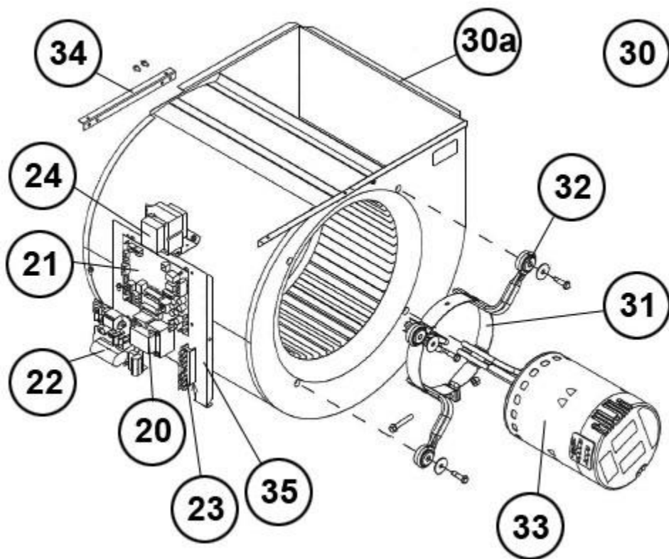
Blower Assembly
