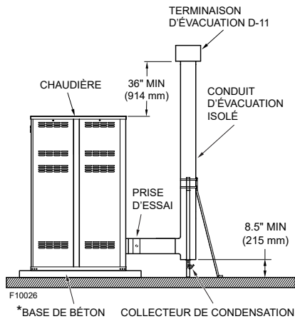
Figure 39. Installation extérieure
