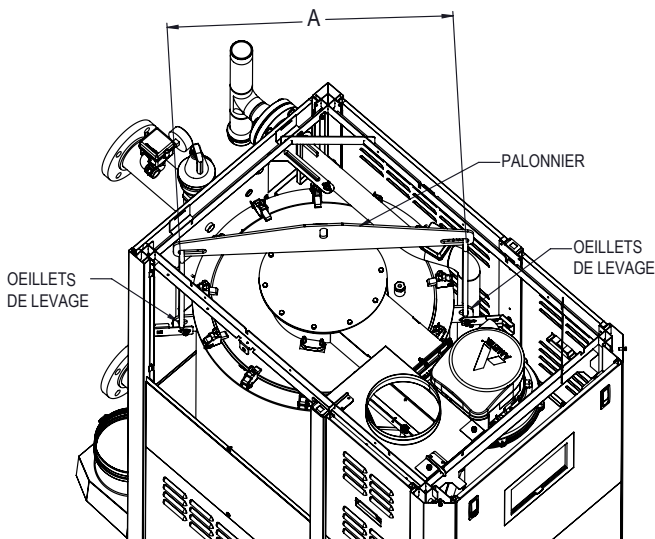
Figure 9. Oeilleets de levage
