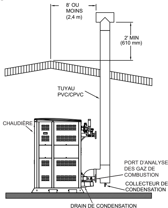
Figure 68. PVC/CPVC - Ventilation verticale
