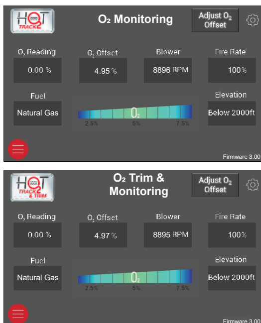
Figure 100. HO2T Track et HO2T Track and Trim
