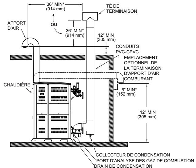
Figure 69. PVC/CPVC - Ventilation directe verticale
