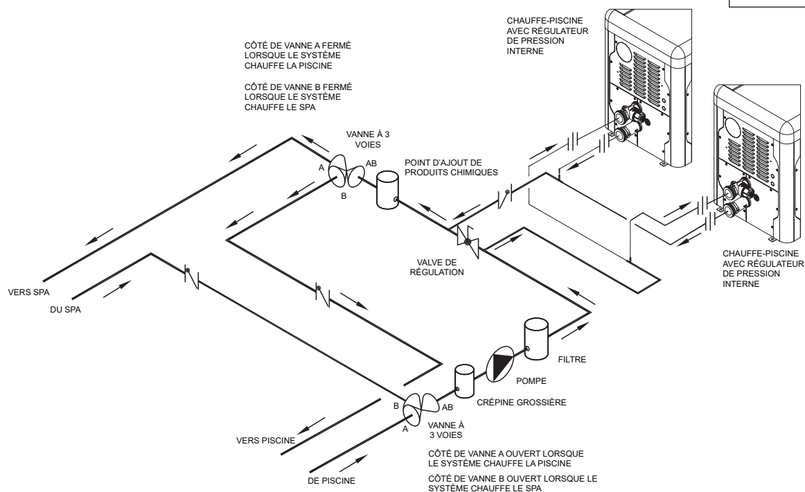
Figure 25. Installation, multi-appareils de chauffage
