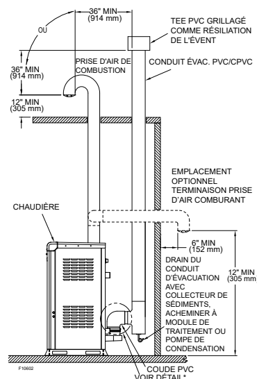
Figure 47. PVC/CPVC - Ventilation directe verticale
