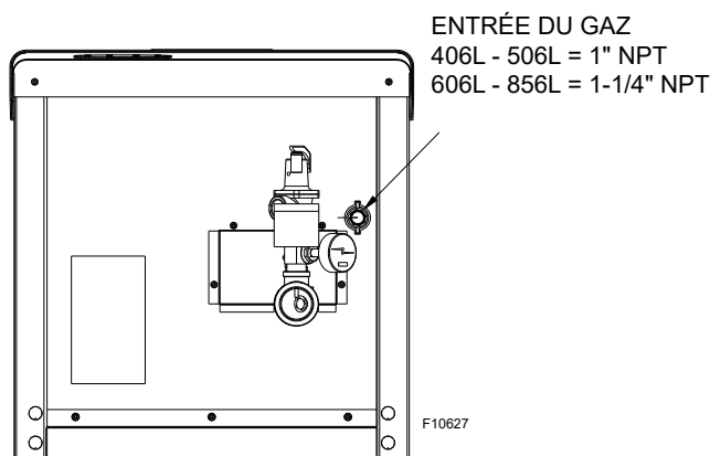
Figure 30. Raccordement du gaz
