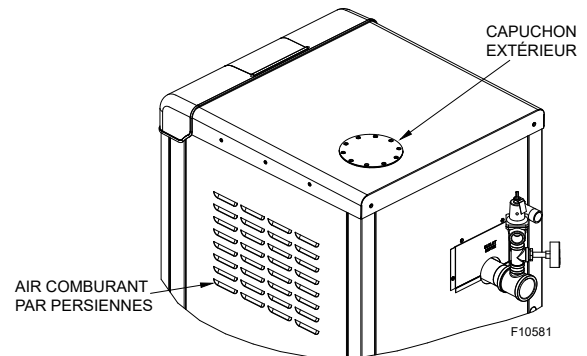
Figure 11. Air comburant, installation extérieure
