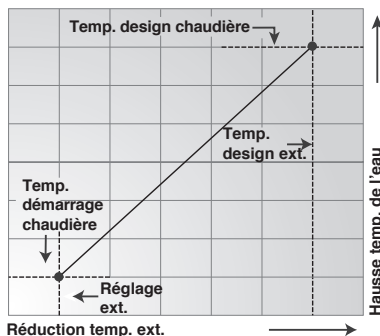
Figure 79. Ratio de compensation
