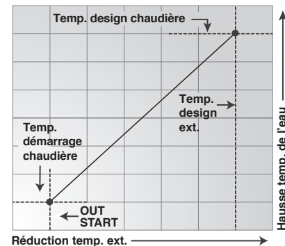
Figure 42. Ratio de compensation
