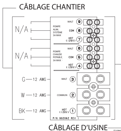
Figure 26. Chaudière asservie
