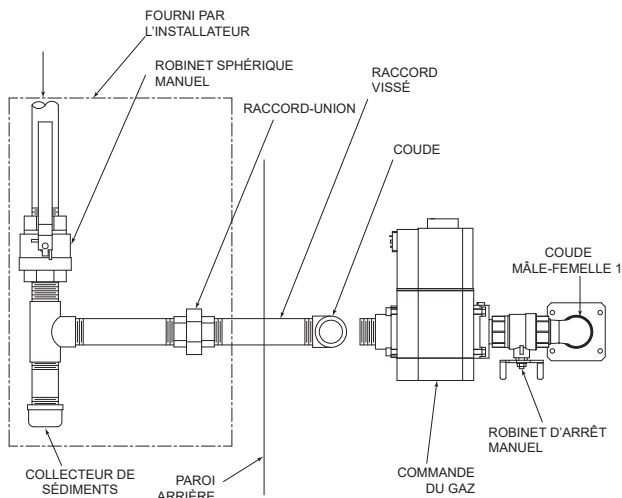
Figure 19. Raccordement du gaz
