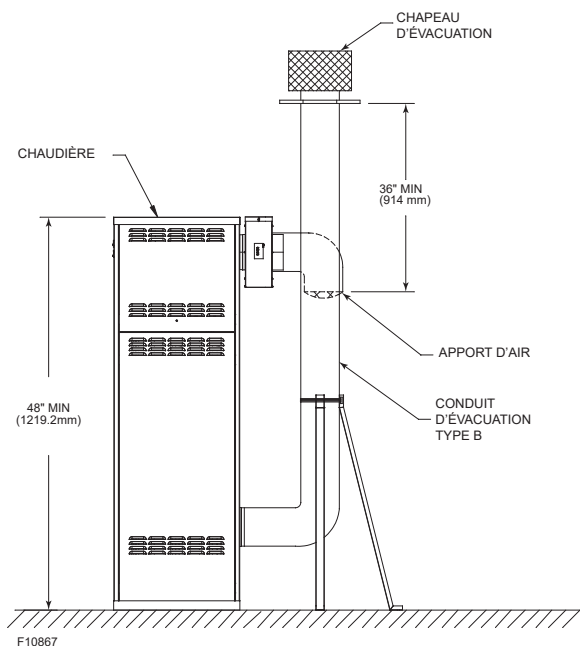
Figure 34. Installation extérieure
