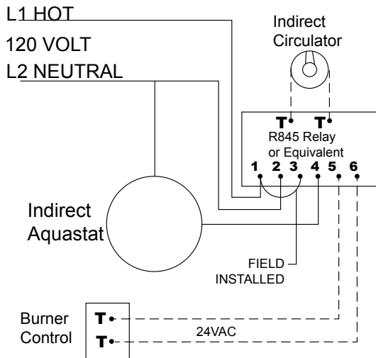
Figure 8. Boiler
