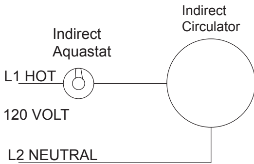
Figure 7. Boiler Maintaining 180°F (82°C)
