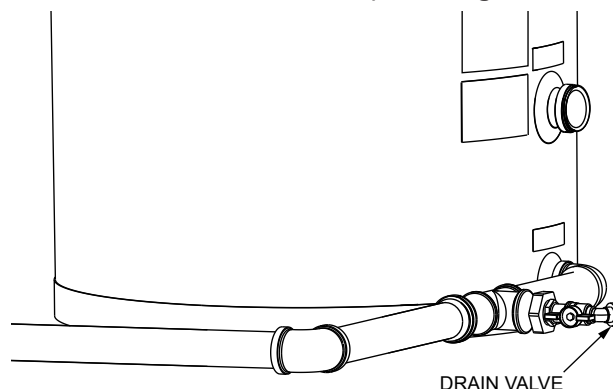
Figure 2. Drain Valve Installation
