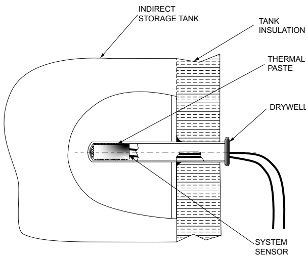
Figure 5. 10 kOhm Thermistor Installation
