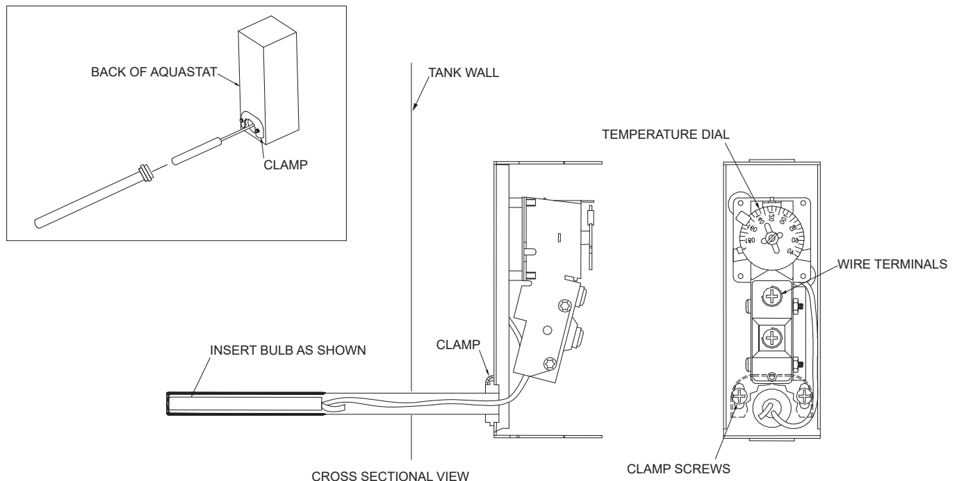
Figure 6. Aquastat Well UNCONTROLLED DOCUMENT IF PRINTED
