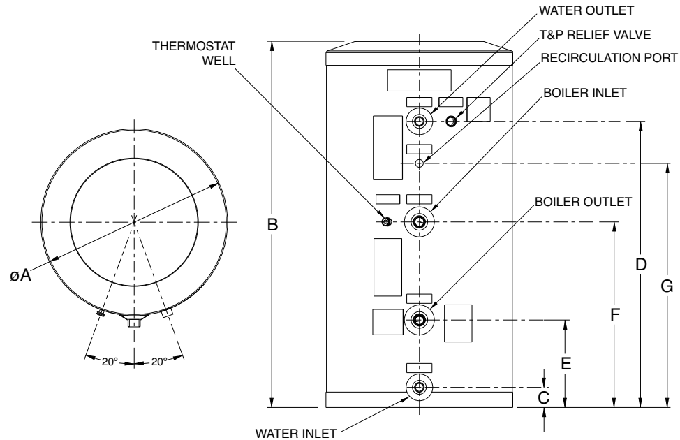
Figure 1. Indirect Water Temperature Dimensions
