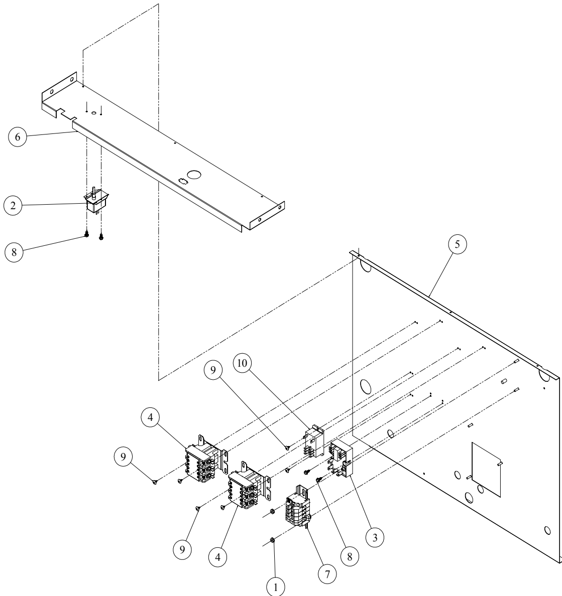
HEATER SHIELD ASM - 03054Z26
