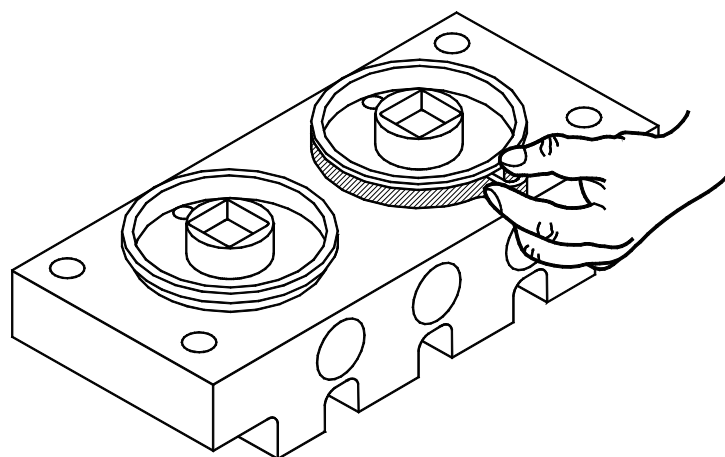
Fig. 8 Front Plate Gasket Removal
