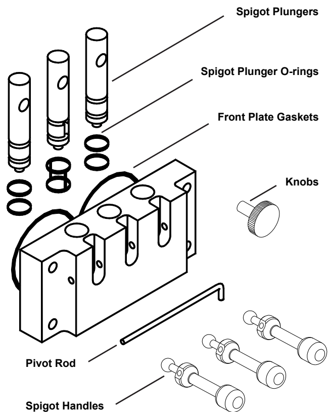
Fig. 14 Front Plate Assembly
