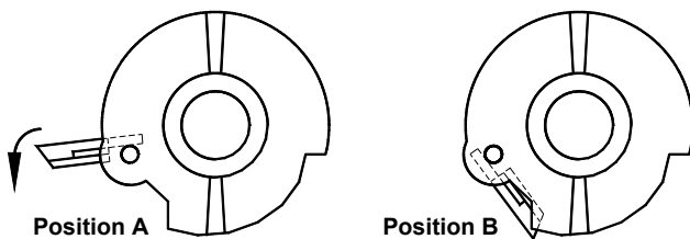
Fig. 18 Dasher (Front View)
