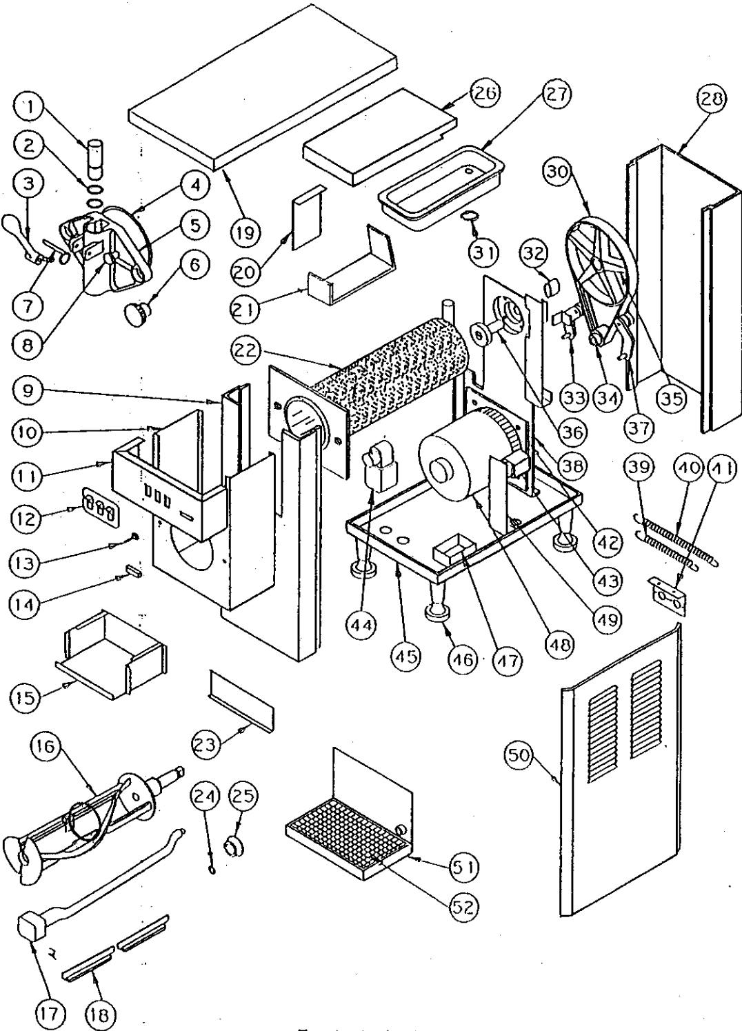
Exploded View
