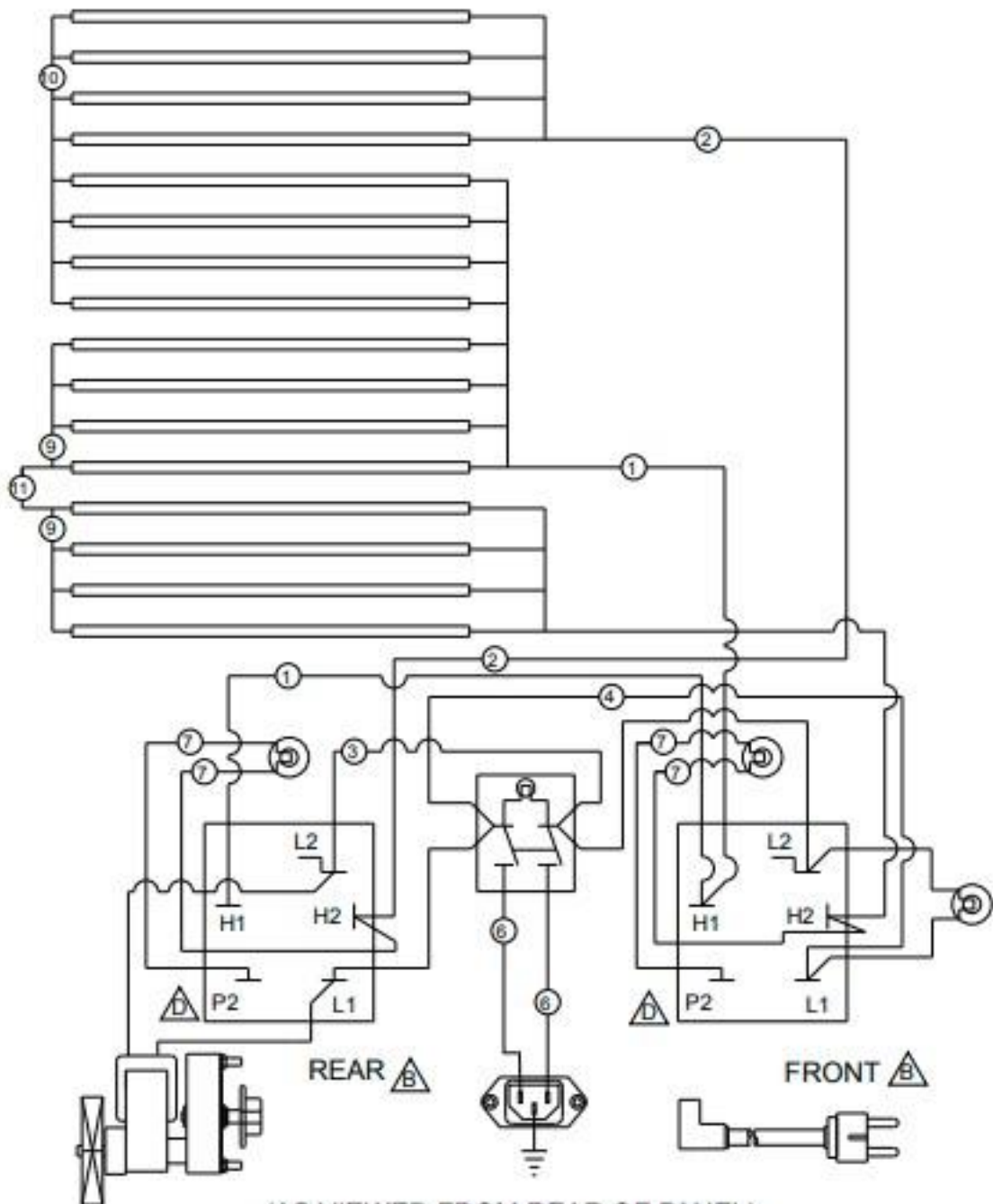
(AS VIEWED FROM REAR OF PANEL)
