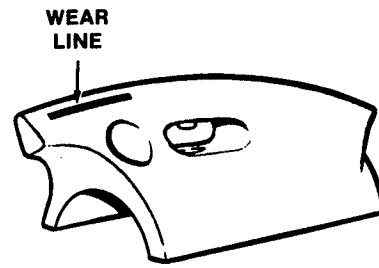
AUGER FLIGHT
