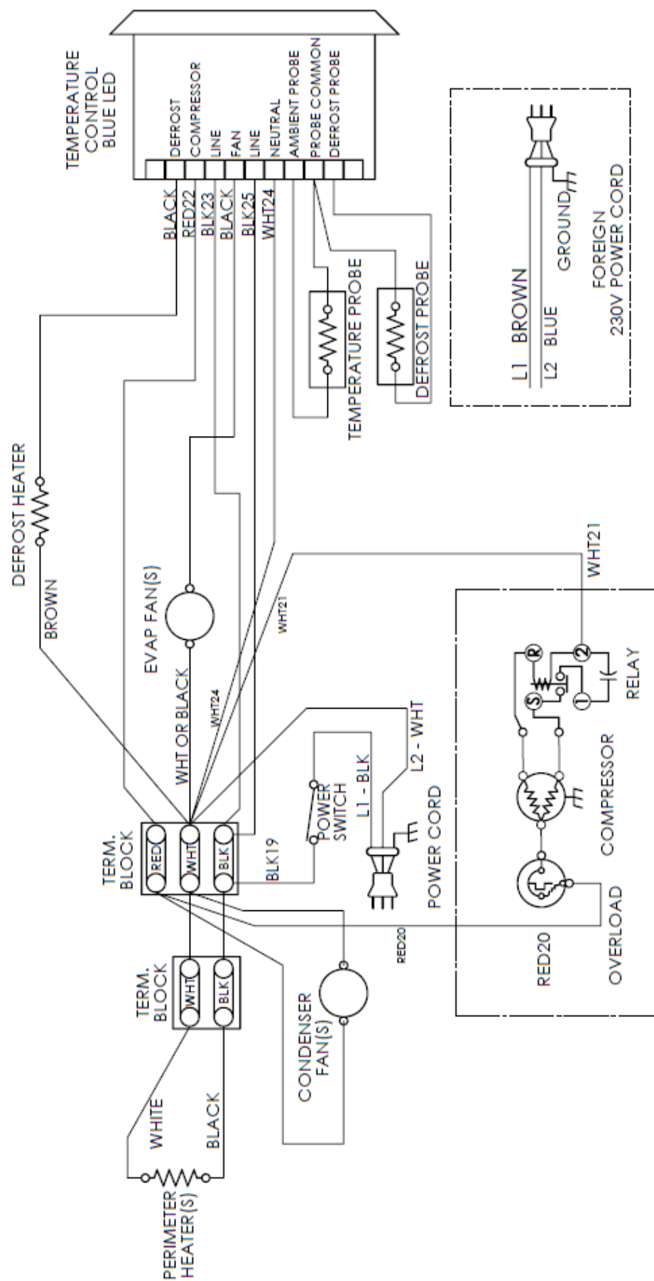
WIRING DIAGRAM 46454 REV A
