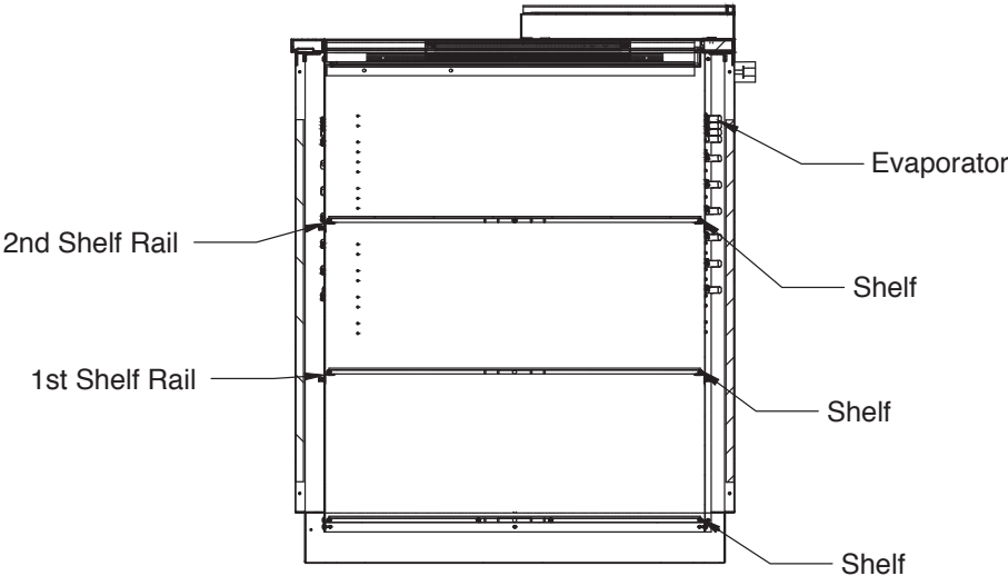
TBC-36S*-GF-N#, TBC-50S*-GF-N#
