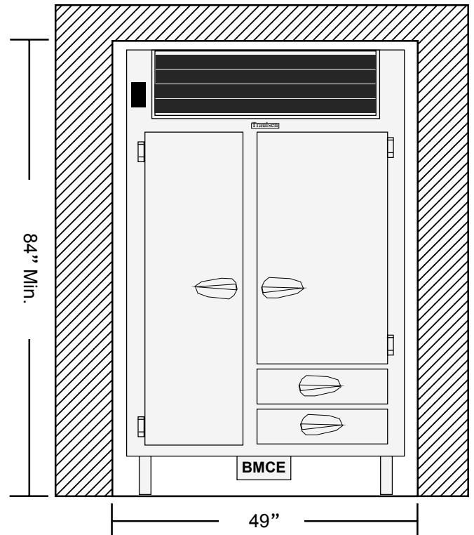
Fig. 4 - Front View Model UR48DT Showing Minimum Built-In Clearances
