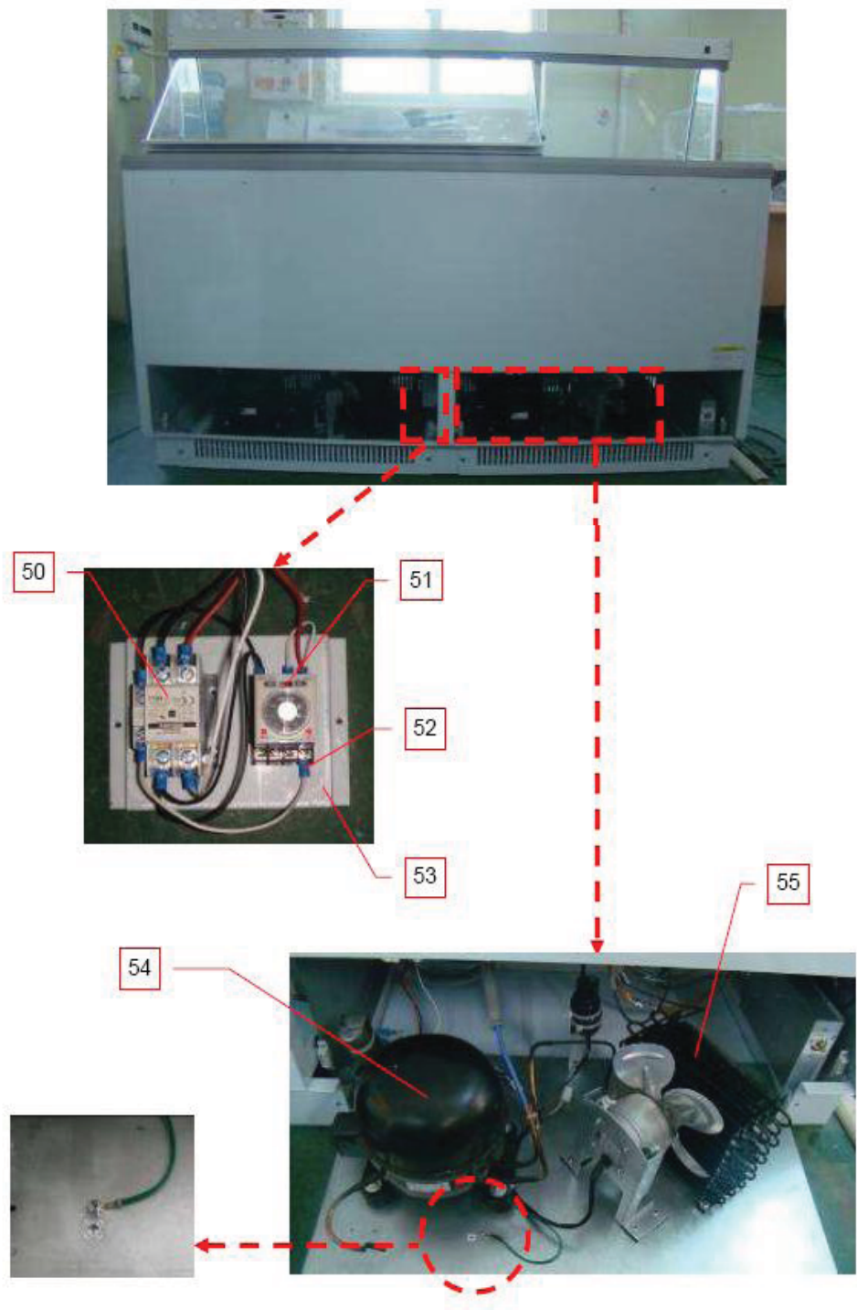
Photo 11 - Machinery compartment view of model TIDC-70W
