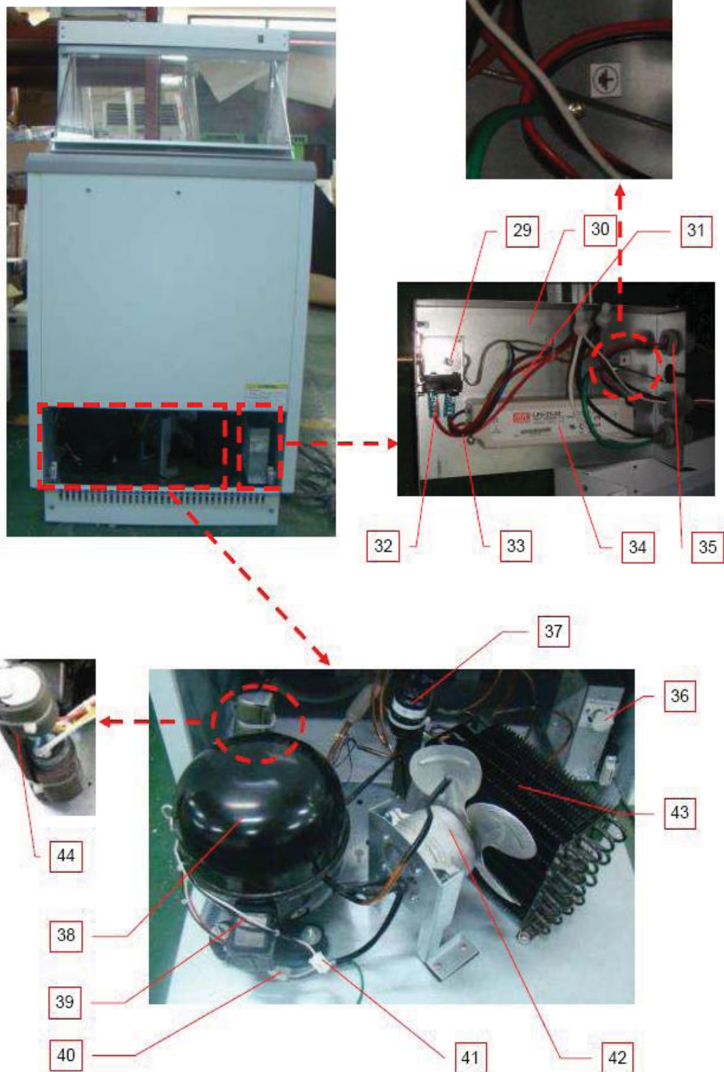
Photo 9 - Machinery compartment view of model TIDC-26W
