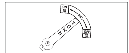
FIGURE 4 BURNER VALVE HANDLE
