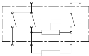
INFINITE CONTROL SCHEMATIC
