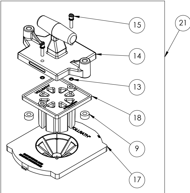
Wedge/Corer Blade Kit
