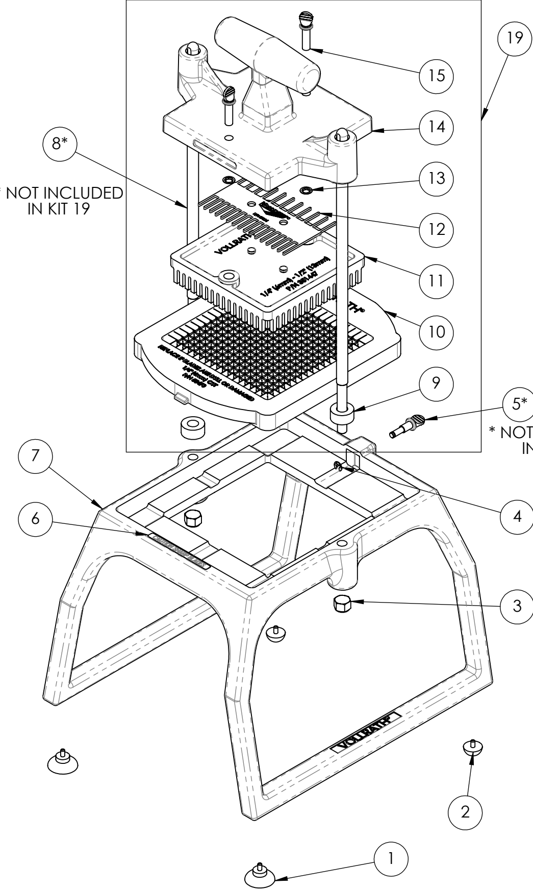
Dice Blade Kit
