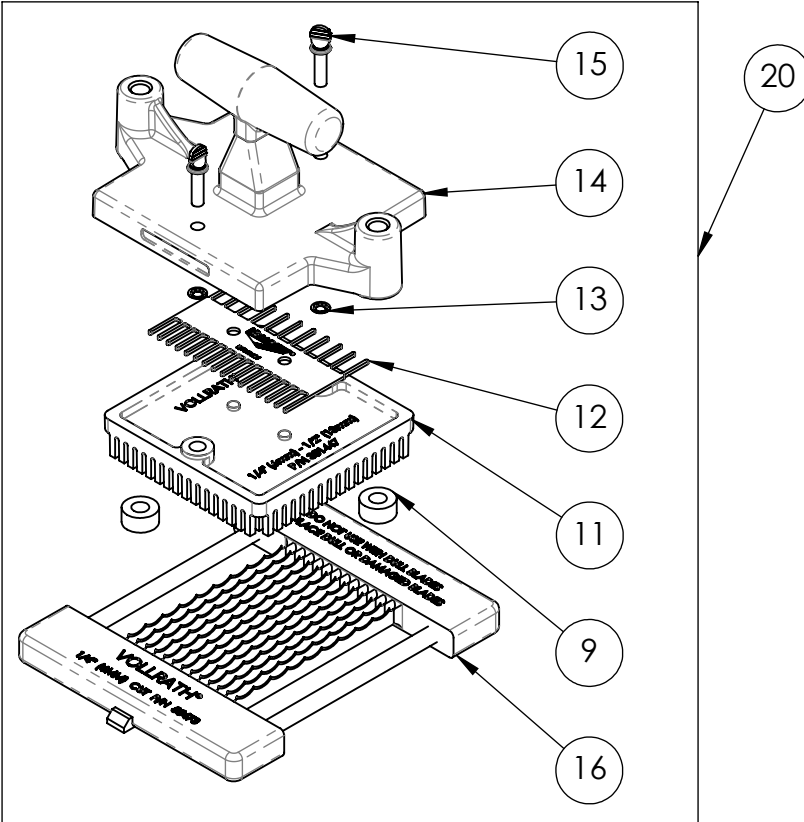
Slice Blade Kit
