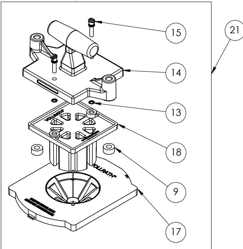
Wedger/Corer Blade Kit
