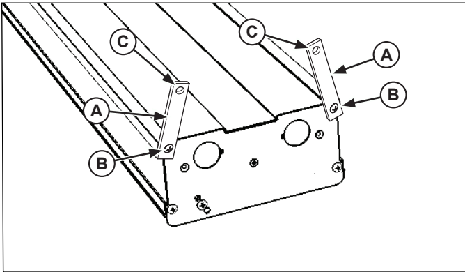
Figure 4. Chain Mount Installation.
