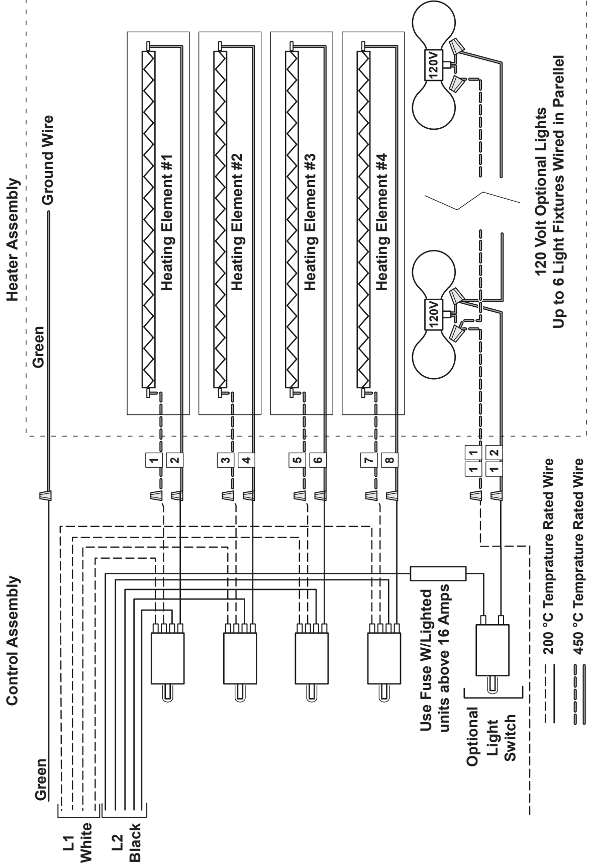
208 - 240 Volt Heater W/Toggle Switch Control Assembly Wiring Diagram
