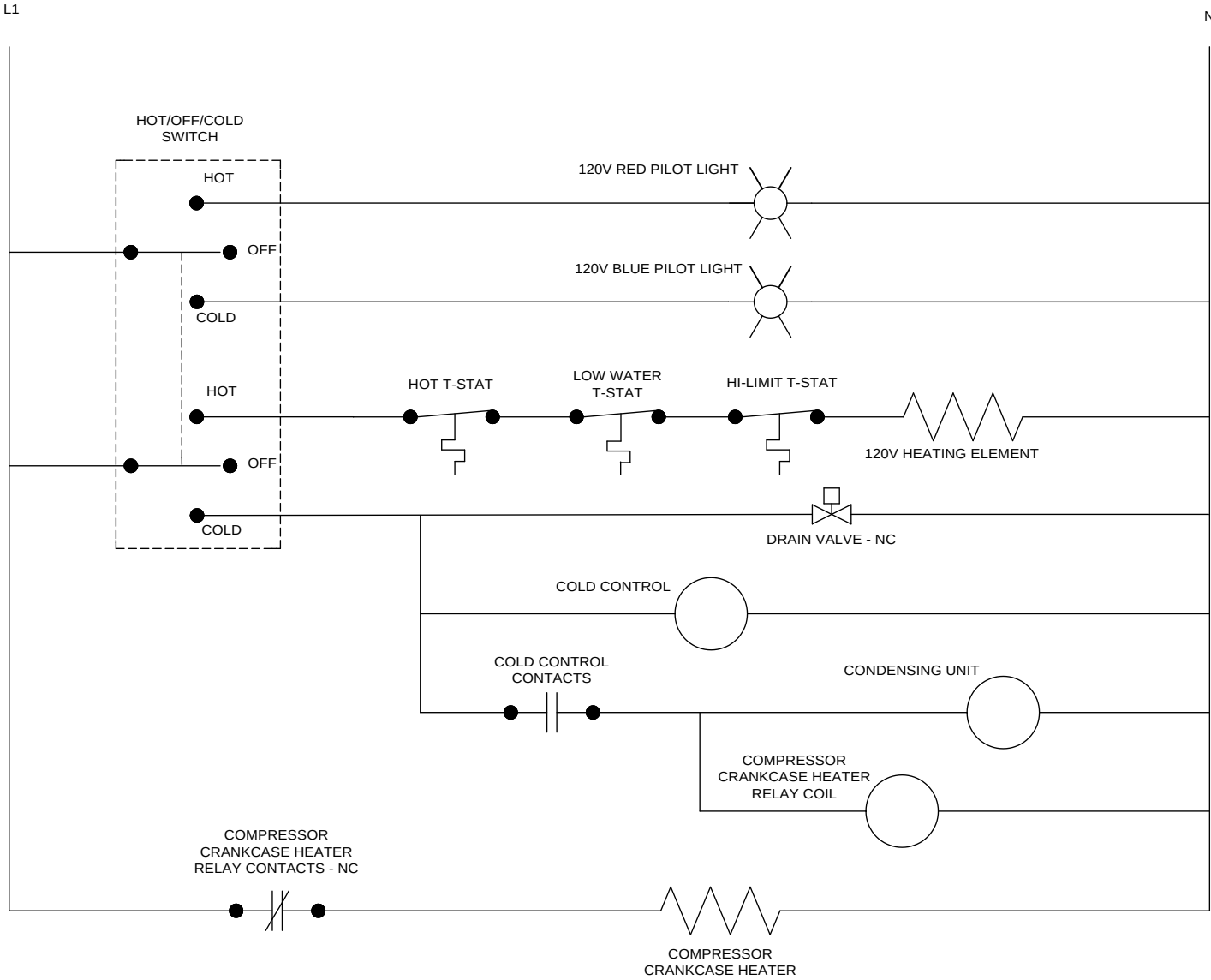
1 WELL HOT & COLD 120V LADDER LOGIC DIAGRAM
