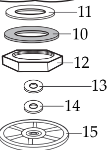
502968 Blending Assy.
