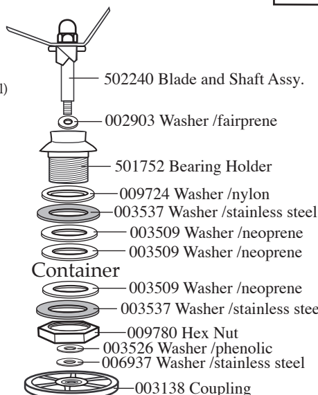
501832 Blending Assy.
