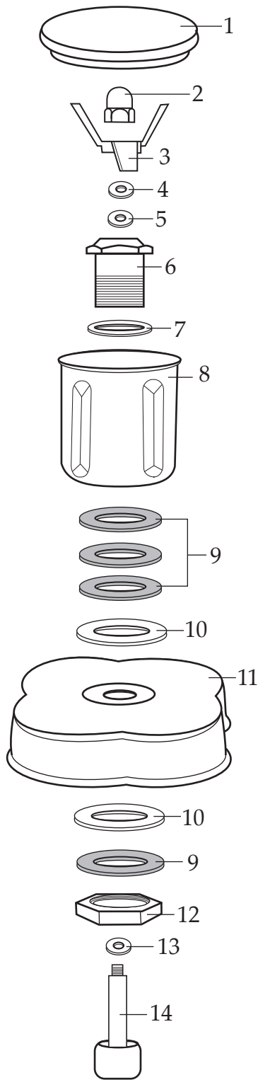
MC1 500132 Blending Assembly
