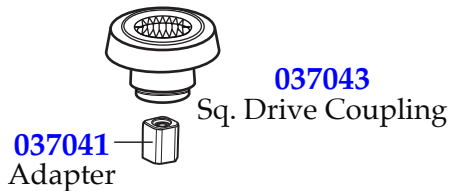
037041 Adapter 037043 Sq. Drive Coupling 503601 Sq. Drive Coupling with Adapter
