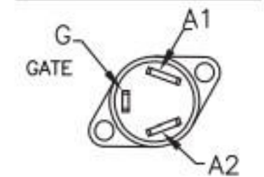
TRIAC PIN ASSIGNMENTS
