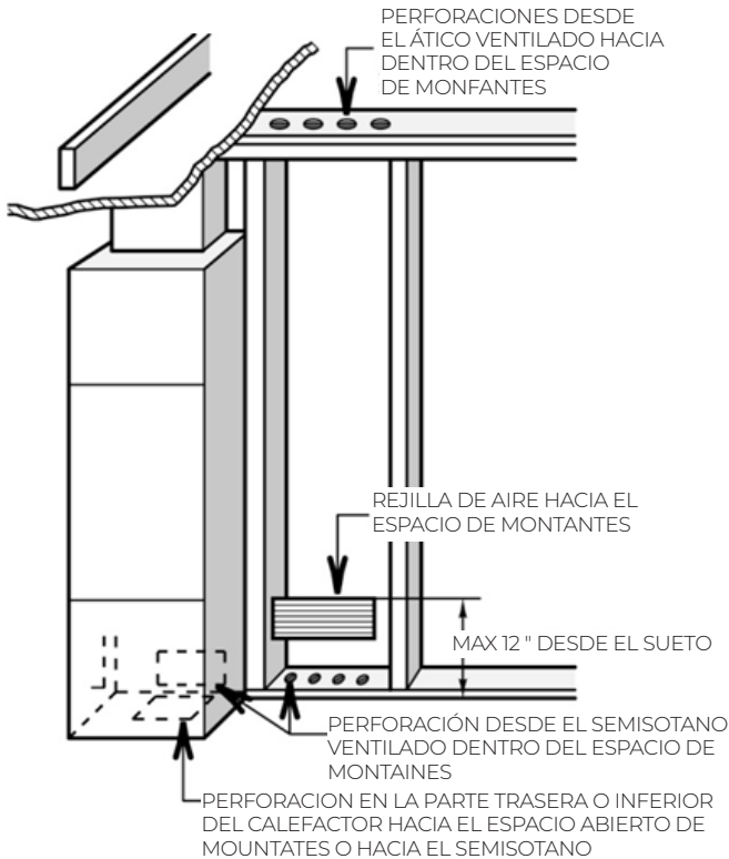
FIGURE 7 - FRESH AIR DUCT
