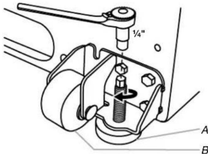
A. Leveling screw B. Front roller
