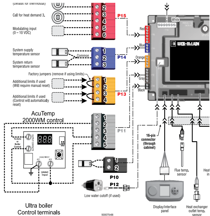
Figure 24 Wiring tank control to the Ultra (1176-100) boiler control.
