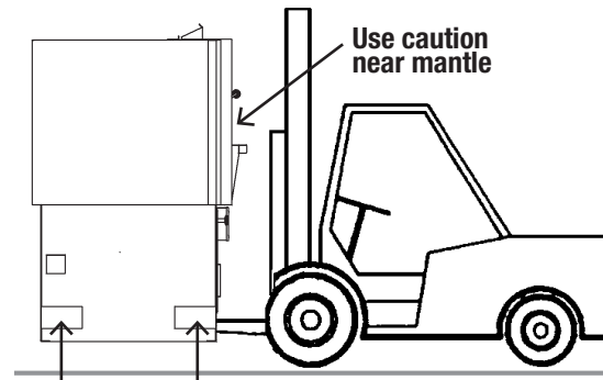
Side Forklift Pockets
